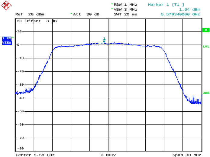
Maximum Power Spectral Density_TNVN_11N20_5580_Ant2
