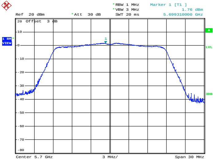
Maximum Power Spectral Density_TNVN_11N20_5700_Ant2
