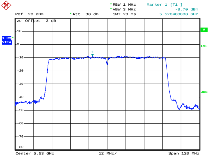
Maximum Power Spectral Density_TNVN_11AC80_5530_Ant2
