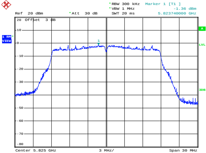
Maximum Power Spectral Density_TNVN_11N20_5825_Ant2
