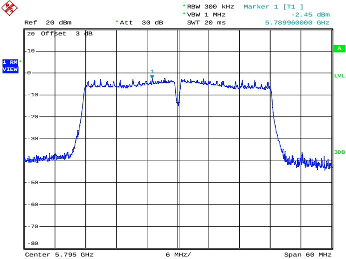
Maximum Power Spectral Density_TNVN_11N40_5795_Ant2
