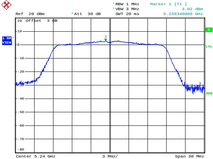
Maximum Power Spectral Density_TNVN_11N20_5240_Ant2
