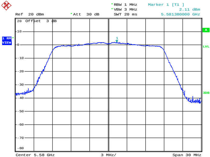
Maximum Power Spectral Density_TNVN_11AC20_5580_Ant2
