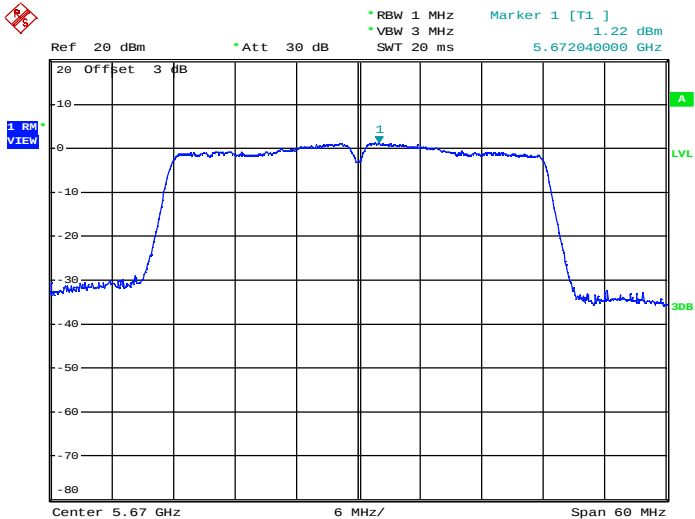
Maximum Power Spectral Density_TNVN_11AC40_5670_Ant2
