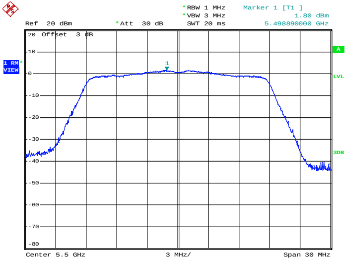
Maximum Power Spectral Density_TNVN_11AC20_5500_Ant2
