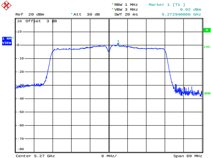
Maximum Power Spectral Density_TNVN_11N40_5270_Ant2
