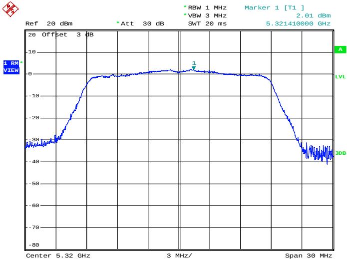
Maximum Power Spectral Density_TNVN_11N20_5320_Ant2
