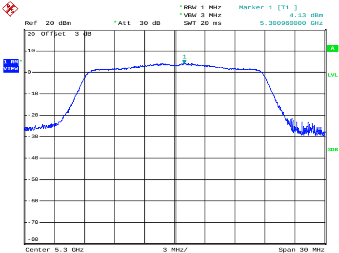
Maximum Power Spectral Density_TNVN_11AC20_5300_Ant2
