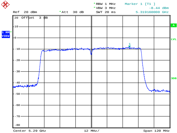
Maximum Power Spectral Density_TNVN_11AC80_5290_Ant2
