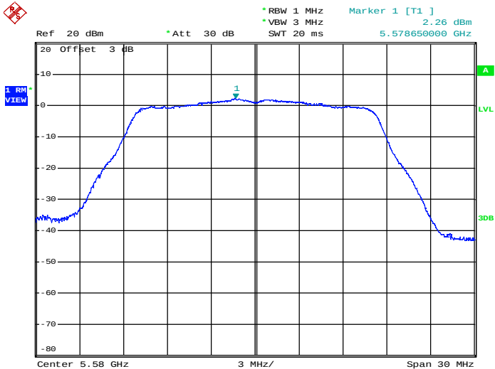
Maximum Power Spectral Density_TNVN_11A_5580_Ant2
