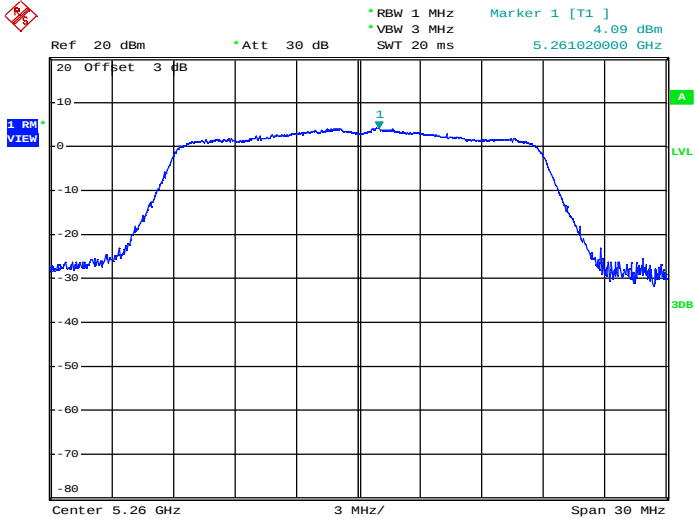
Maximum Power Spectral Density_TNVN_11N20_5260_Ant2
