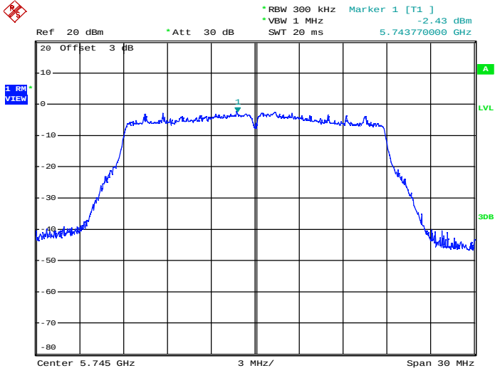
Maximum Power Spectral Density_TNVN_11AC20_5745_Ant2
