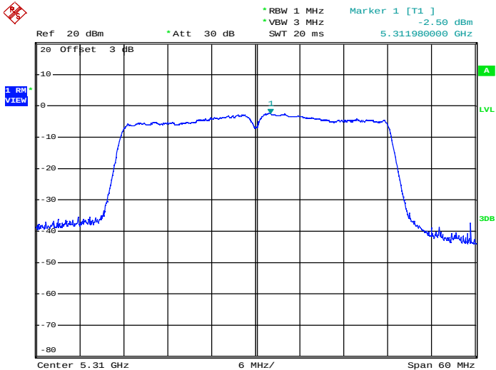
Maximum Power Spectral Density_TNVN_11N40_5310_Ant2
