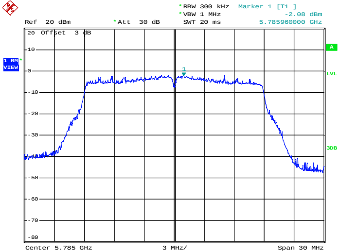
Maximum Power Spectral Density_TNVN_11AC20_5785_Ant2
