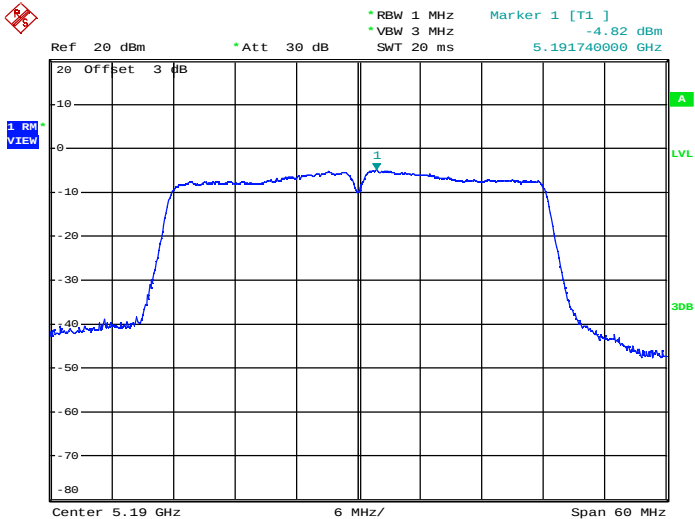
Maximum Power Spectral Density_TNVN_11N40_5190_Ant2
