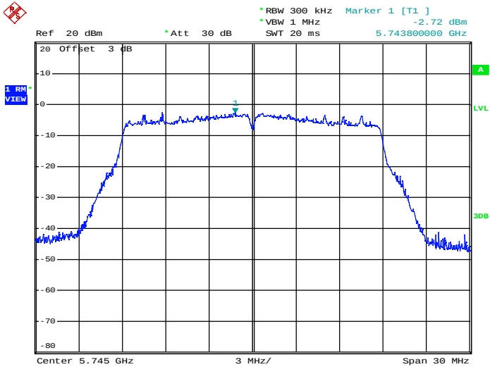
Maximum Power Spectral Density_TNVN_11N20_5745_Ant2
