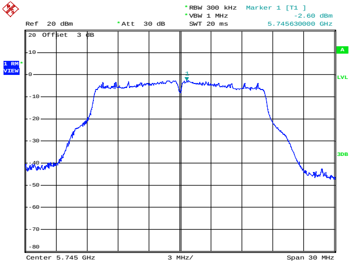
Maximum Power Spectral Density_TNVN_11A_5745_Ant2
