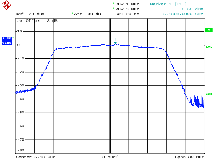
Maximum Power Spectral Density_TNVN_11AC20_5180_Ant2
