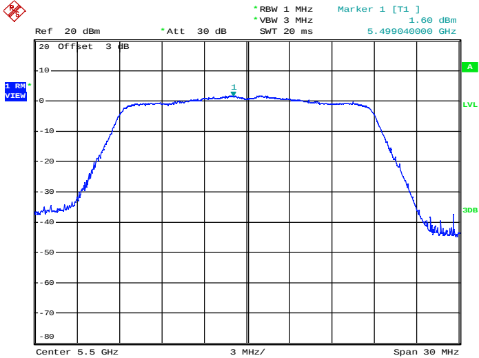
Maximum Power Spectral Density_TNVN_11N20_5500_Ant2
