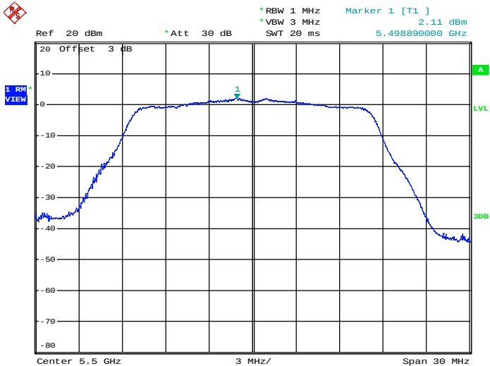
Maximum Power Spectral Density_TNVN_11A_5500_Ant2
