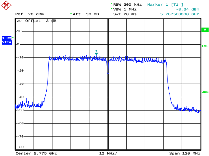
Maximum Power Spectral Density_TNVN_11AC80_5775_Ant2
