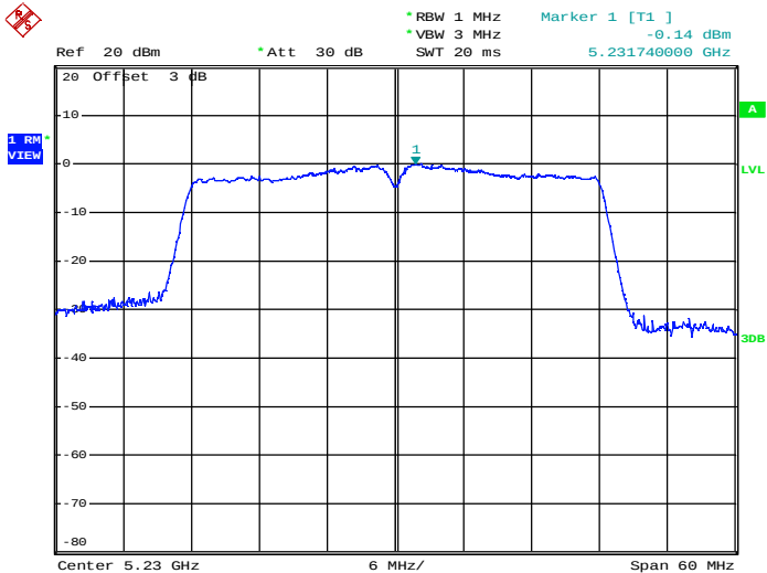
Maximum Power Spectral Density_TNVN_11AC40_5230_Ant2
