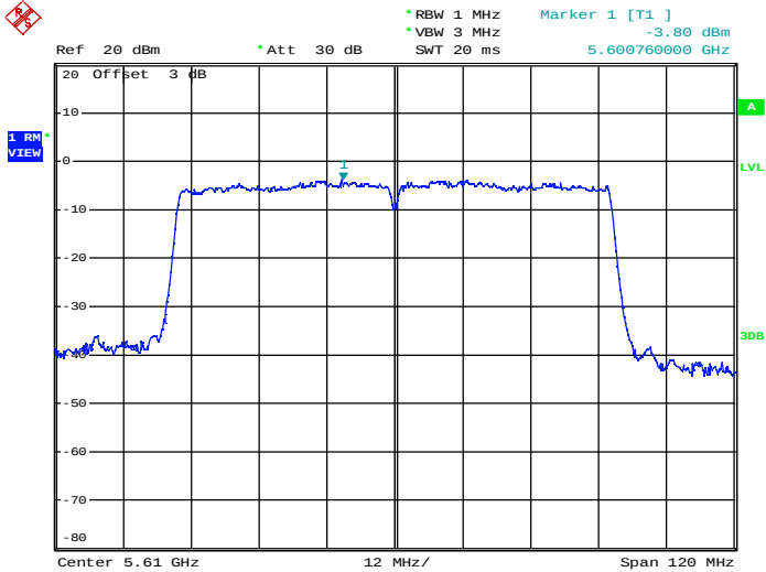
Maximum Power Spectral Density_TNVN_11AC80_5610_Ant2
