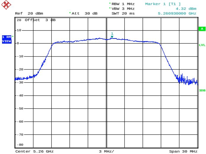
Maximum Power Spectral Density_TNVN_11AC20_5260_Ant2
