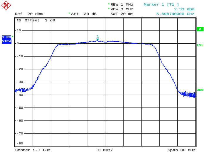
Maximum Power Spectral Density_TNVN_11A_5700_Ant2
