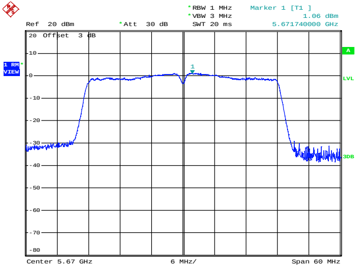
Maximum Power Spectral Density_TNVN_11N40_5670_Ant2
