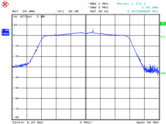
Maximum Power Spectral Density_TNVN_11AC20_5240_Ant2
