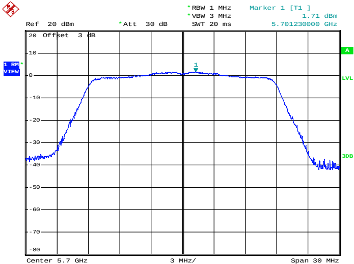
Maximum Power Spectral Density_TNVN_11AC20_5700_Ant2
