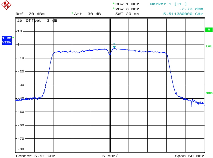
Maximum Power Spectral Density_TNVN_11AC40_5510_Ant2
