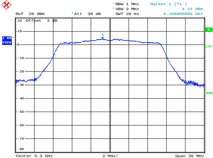
Maximum Power Spectral Density_TNVN_11A_5300_Ant2
