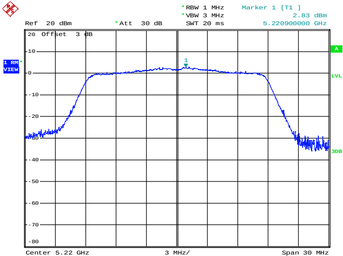
Maximum Power Spectral Density_TNVN_11AC20_5220_Ant2
