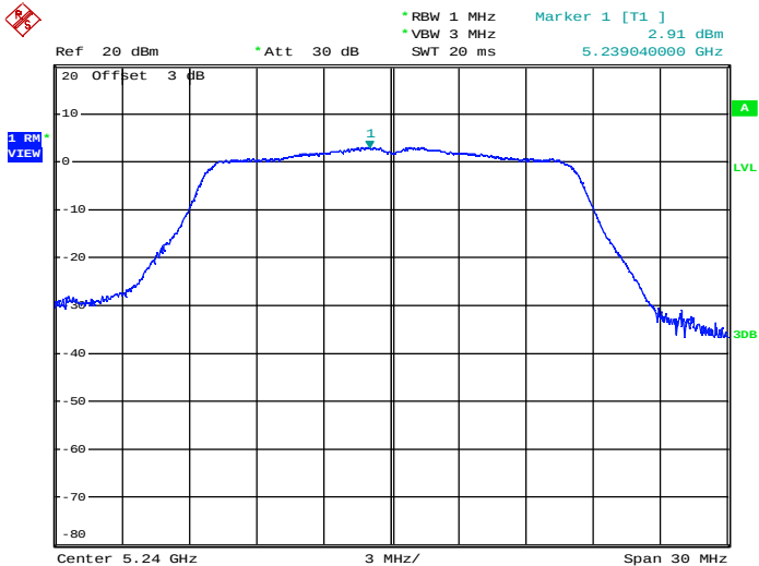
Maximum Power Spectral Density_TNVN_11A_5240_Ant2
