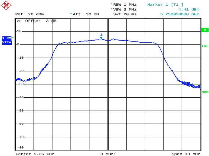
Maximum Power Spectral Density_TNVN_11A_5260_Ant2
