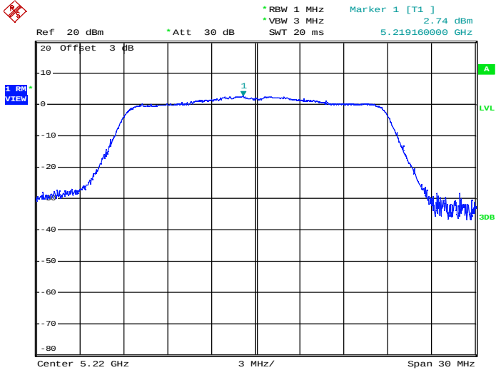
Maximum Power Spectral Density_TNVN_11N20_5220_Ant2
