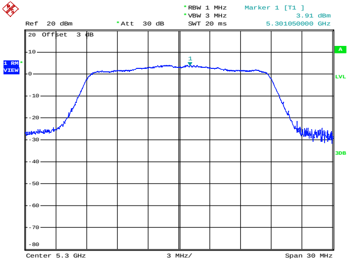
Maximum Power Spectral Density_TNVN_11N20_5300_Ant2
