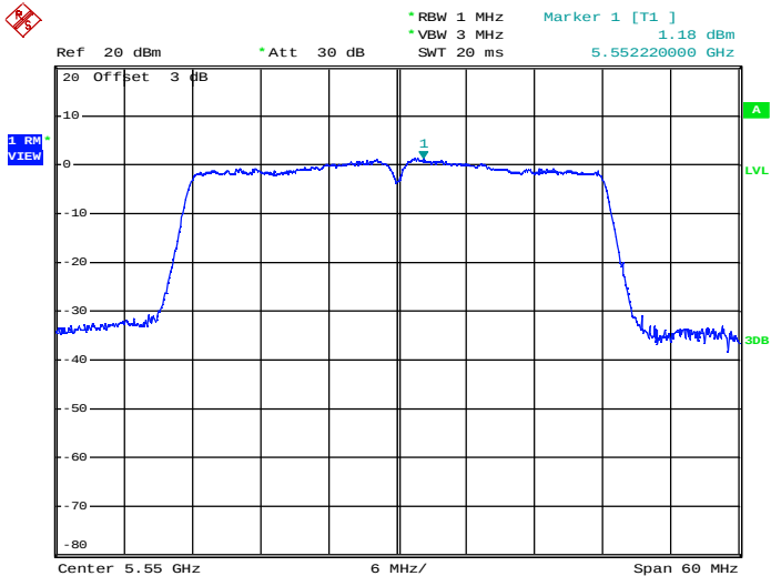
Maximum Power Spectral Density_TNVN_11AC40_5550_Ant2
