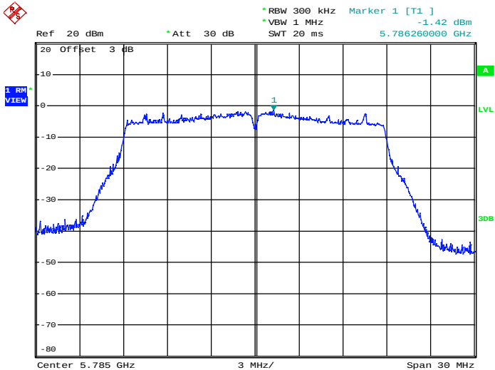
Maximum Power Spectral Density_TNVN_11N20_5785_Ant2
