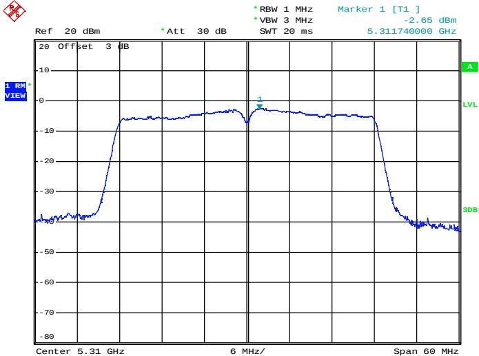
Maximum Power Spectral Density_TNVN_11AC40_5310_Ant2
