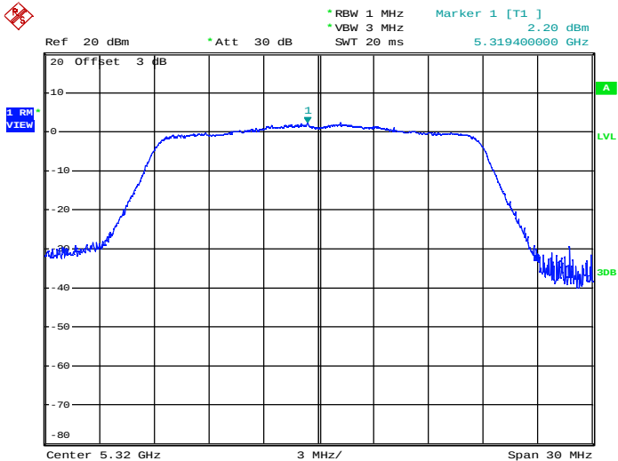
Maximum Power Spectral Density_TNVN_11AC20_5320_Ant2
