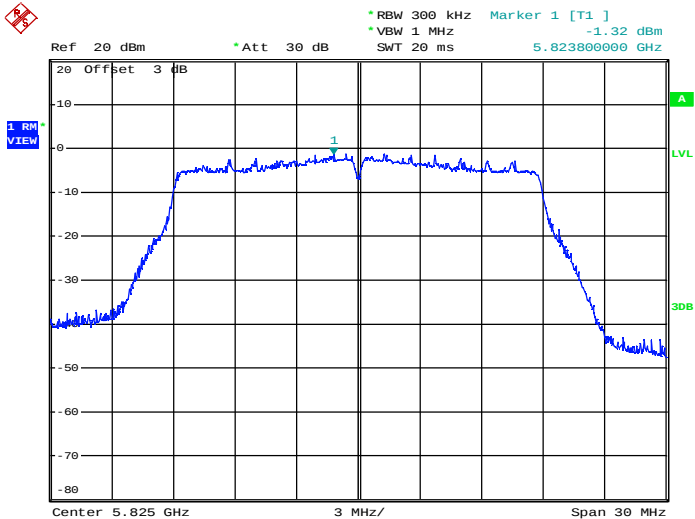
Maximum Power Spectral Density_TNVN_11AC20_5825_Ant2
