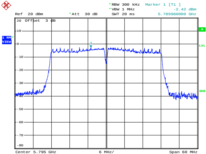
Maximum Power Spectral Density_TNVN_11AC40_5795_Ant2
