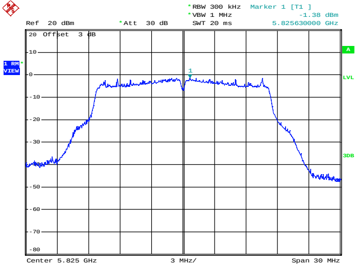
Maximum Power Spectral Density_TNVN_11A_5825_Ant2
