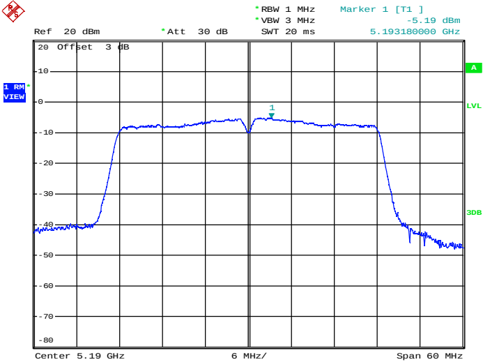
Maximum Power Spectral Density_TNVN_11AC40_5190_Ant2
