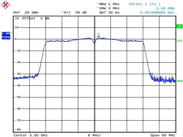
Maximum Power Spectral Density_TNVN_11N40_5550_Ant2
