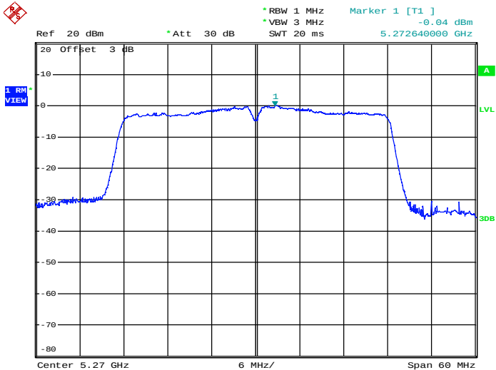
Maximum Power Spectral Density_TNVN_11AC40_5270_Ant2
