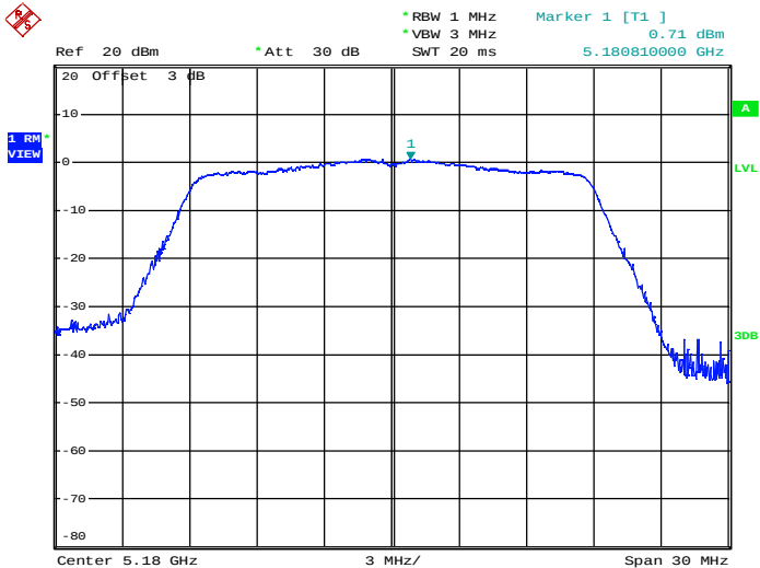
Maximum Power Spectral Density_TNVN_11N20_5180_Ant2
