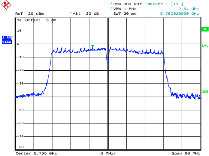
Maximum Power Spectral Density_TNVN_11AC40_5755_Ant2
