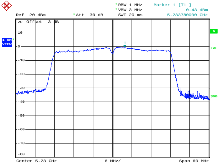
Maximum Power Spectral Density_TNVN_11N40_5230_Ant2
