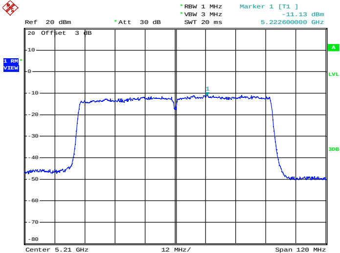
Maximum Power Spectral Density_TNVN_11AC80_5210_Ant2
