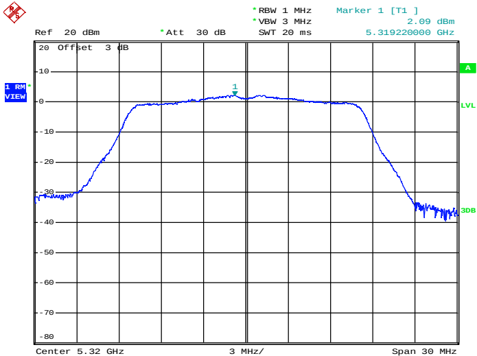
Maximum Power Spectral Density_TNVN_11A_5320_Ant2
