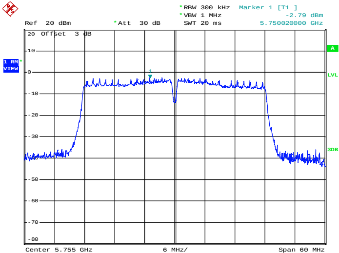
Maximum Power Spectral Density_TNVN_11N40_5755_Ant2
