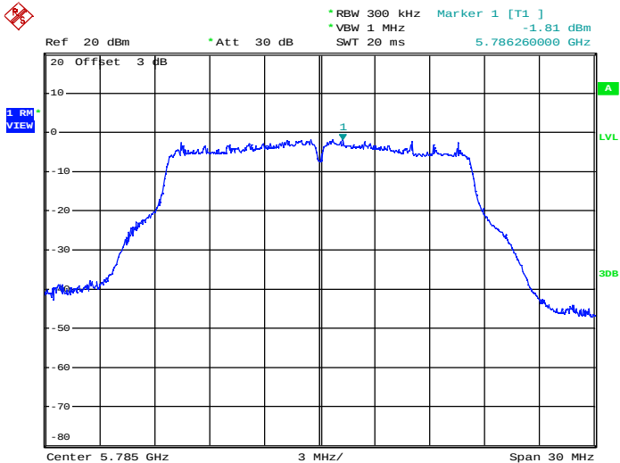
Maximum Power Spectral Density_TNVN_11A_5785_Ant2
