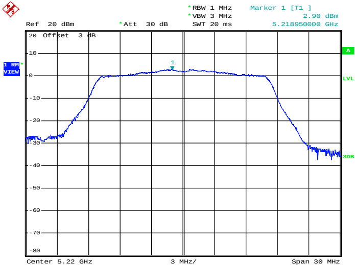
Maximum Power Spectral Density_TNVN_11A_5220_Ant2
