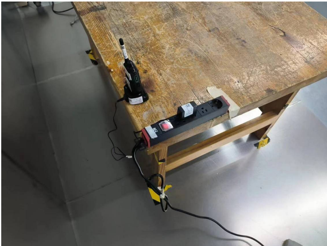
Conducted Emissions Side View –Model AXP695 UHF
