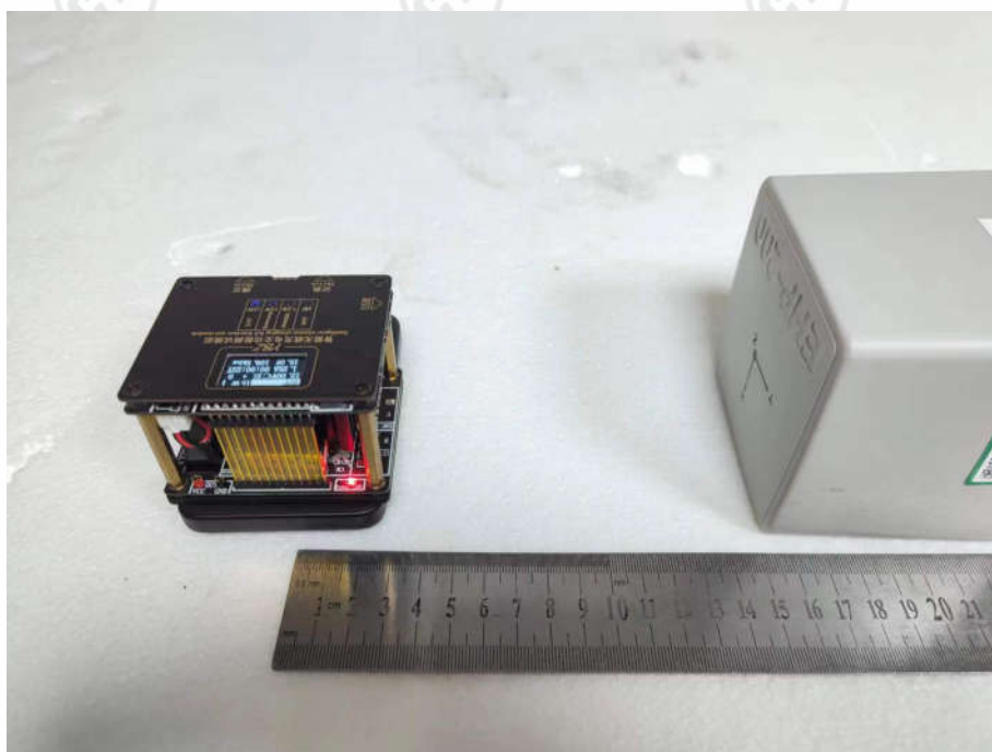
Test Setup of Left (Mode b to Mode e)
