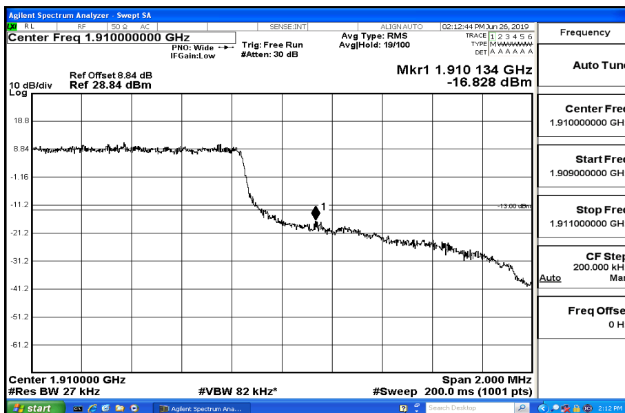
Band Edge Test Graph(s) (Channel Bandwidth: 1.4 MHz)_HCH_QPSK
