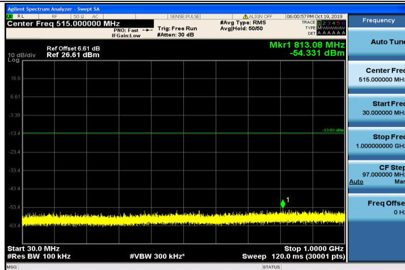
Band4-20MHz-QPSK-20175-1RB#0-30~1000MHz
