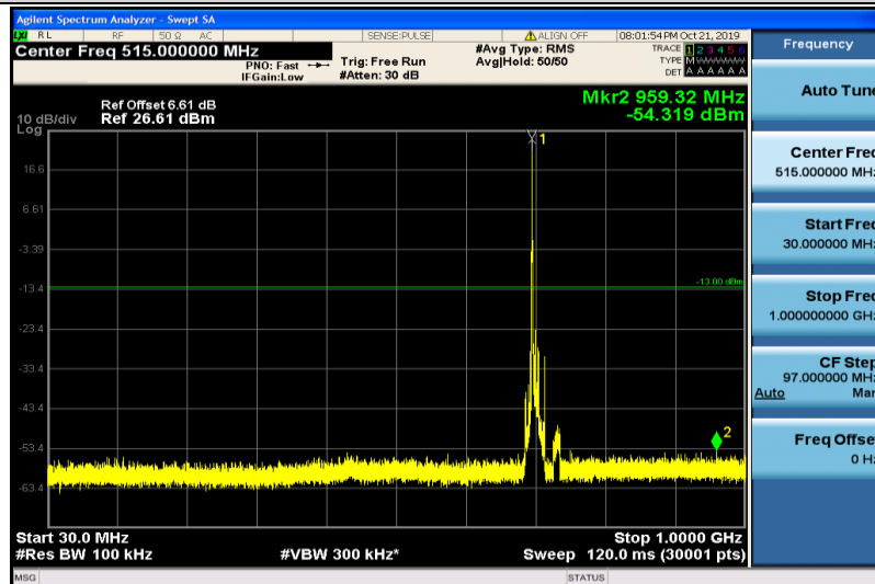
Band12-10MHz-16QAM-23095-1RB#0-30~1000MHz
