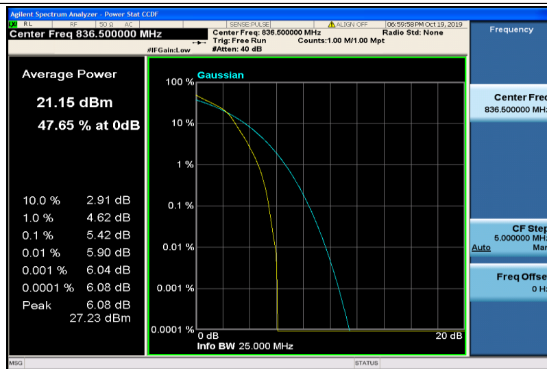
Band5-1.4MHz-16QAM-20525-6RB#0
