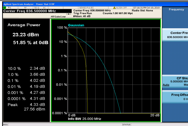
Band5-3MHz-QPSK-20525-1RB#0
