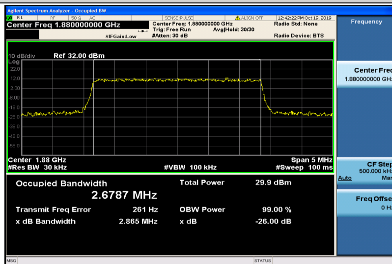
Band2-3MHz-QPSK-18900-15RB#0-2.6787
