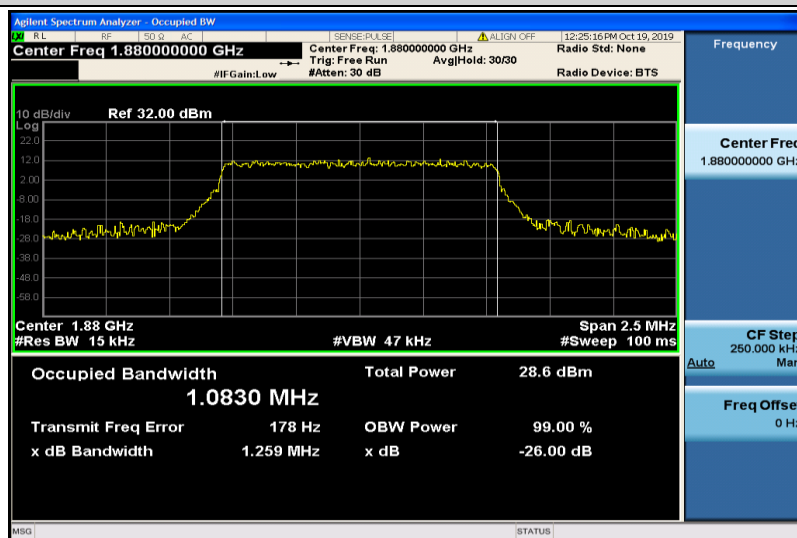
Band2-1.4MHz-16QAM-18900-6RB#0-1.0830
