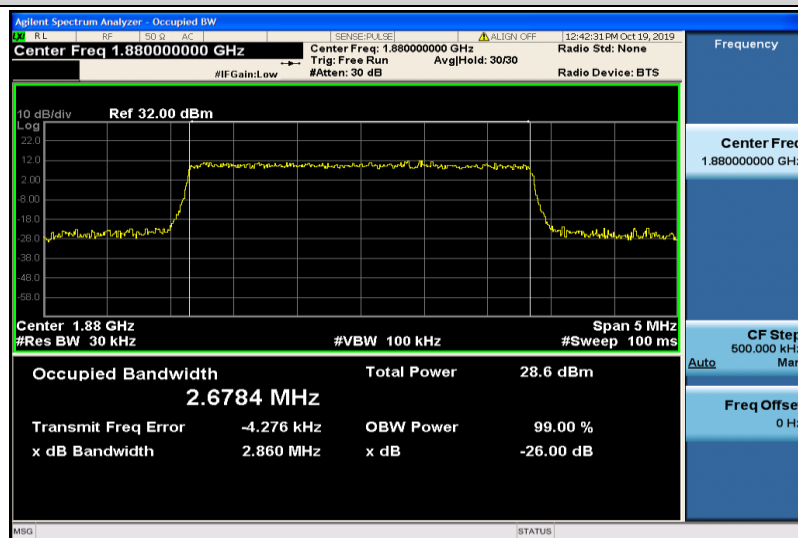
Band2-3MHz-16QAM-18900-15RB#0-2.6784
