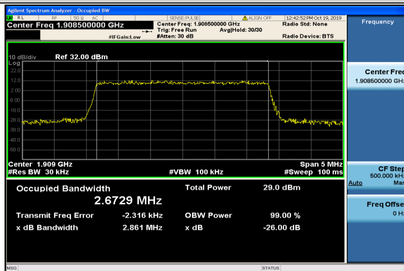
Band2-3MHz-16QAM-19185-15RB#0-2.6729
