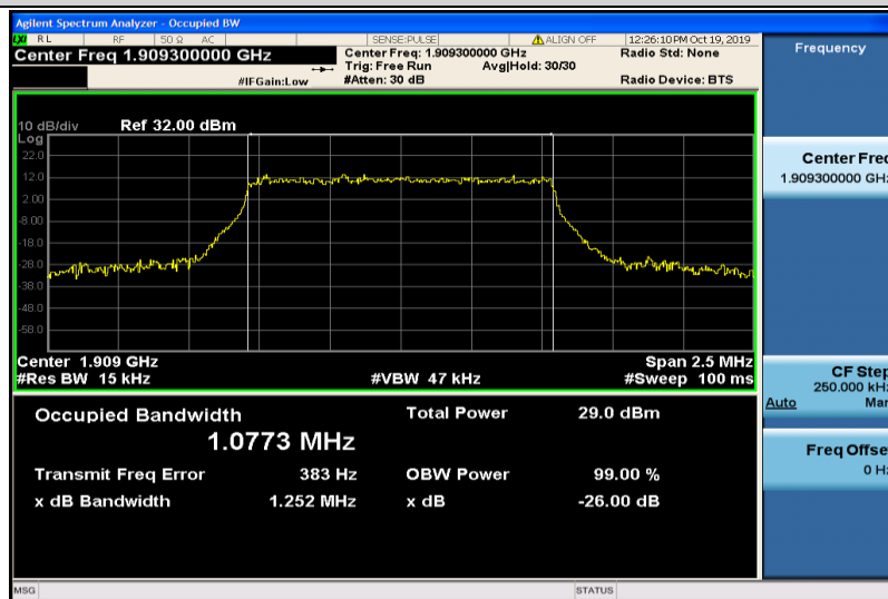
Band2-1.4MHz-16QAM-19193-6RB#0-1.0773
