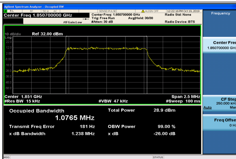
Band2-1.4MHz-16QAM-18607-6RB#0-1.0765
