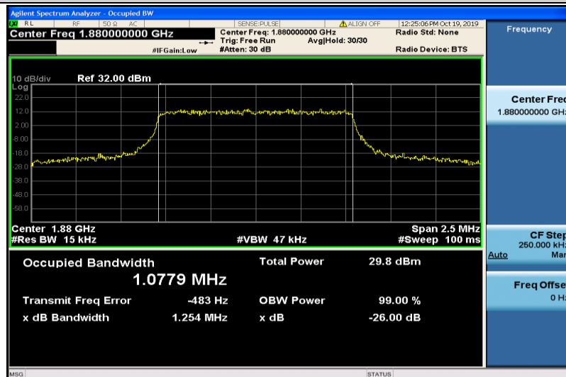
Band2-1.4MHz-QPSK-18900-6RB#0-1.0779
