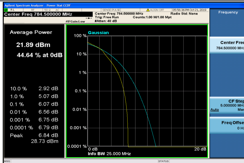
Band13-5MHz-16QAM-23255-25RB#0
