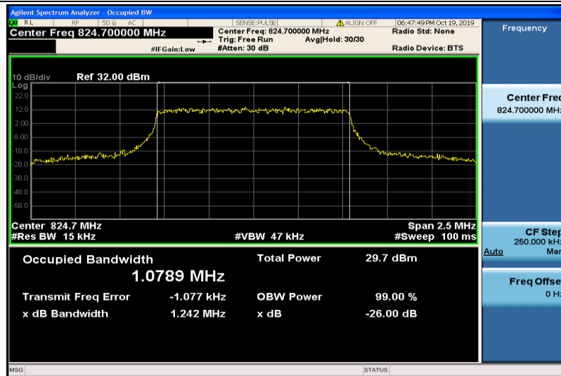
Band5-1.4MHz-QPSK-20407-6RB#0-1.0789
