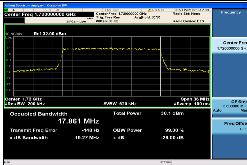
Band4-20MHz-16QAM-20050-100RB#0-17.861
