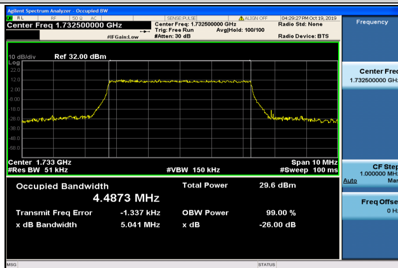
Band4-5MHz-16QAM-20175-25RB#0-4.4873
