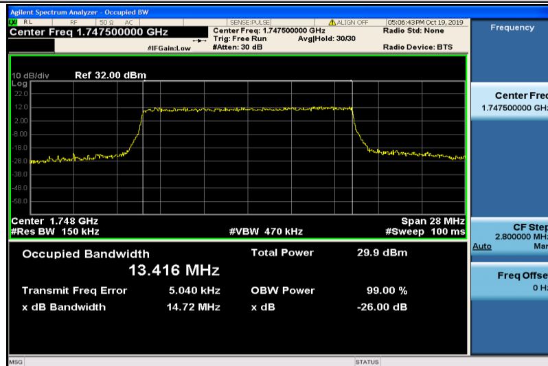
Band4-15MHz-16QAM-20325-75RB#0-13.416
