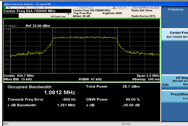
Band5-1.4MHz-16QAM-20407-6RB#0-1.0812
