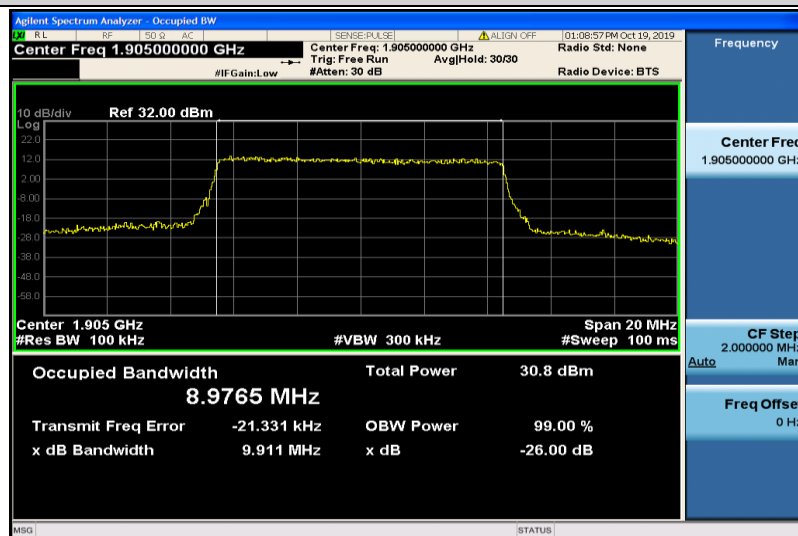
Band2-10MHz-QPSK-19150-50RB#0-8.9765
