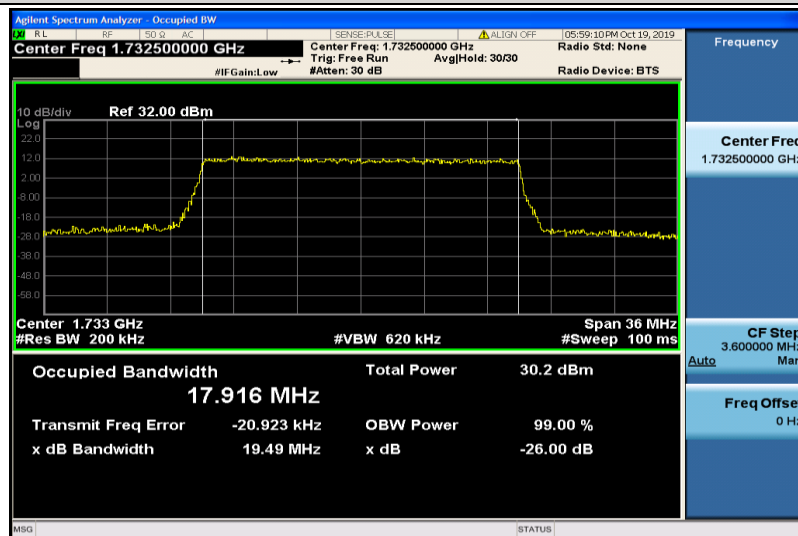
Band4-20MHz-16QAM-20175-100RB#0-17.916
