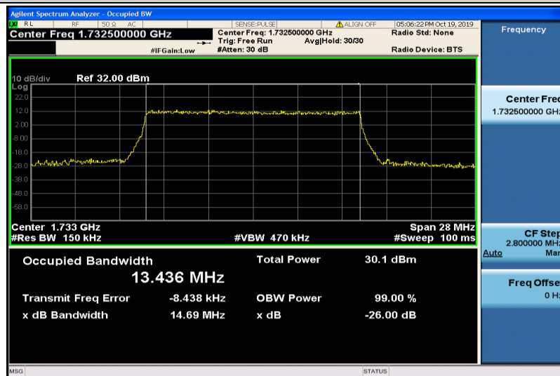
Band4-15MHz-16QAM-20175-75RB#0-13.436
