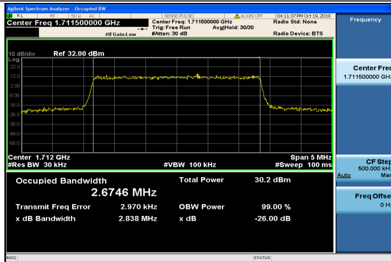
Band4-3MHz-QPSK-19965-15RB#0-2.6746
