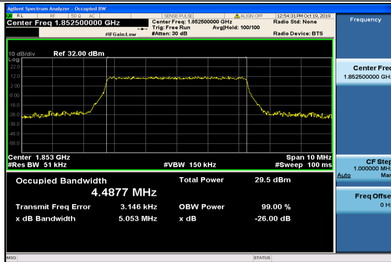
Band2-5MHz-16QAM-18625-25RB#0-4.4877
