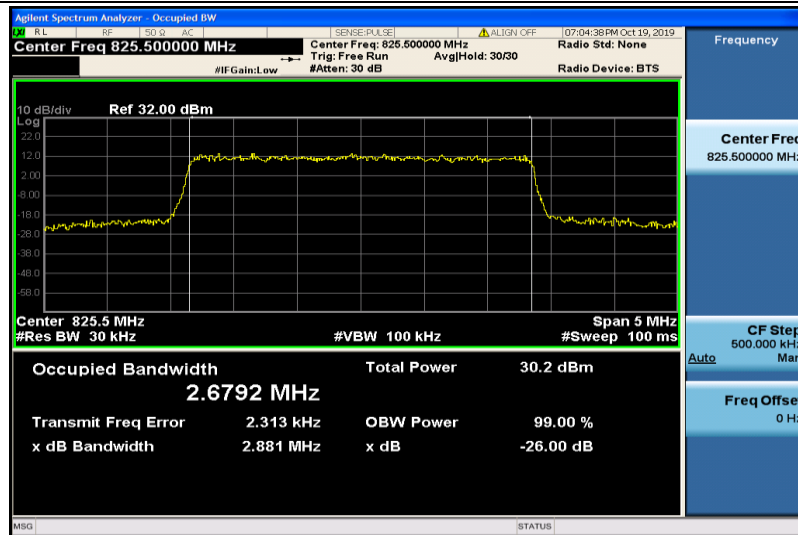
Band5-3MHz-QPSK-20415-15RB#0-2.6792
