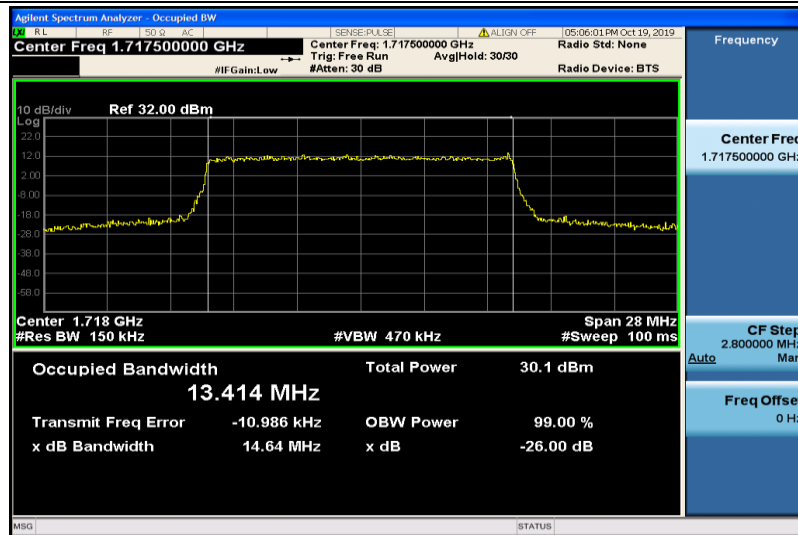
Band4-15MHz-16QAM-20025-75RB#0-13.414
