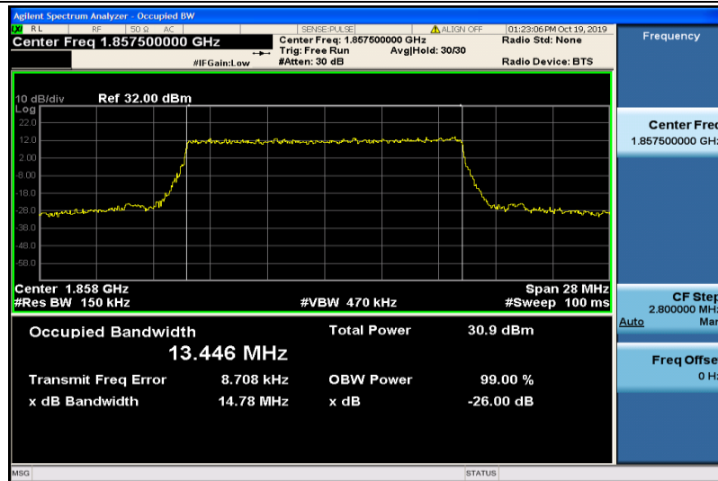
Band2-15MHz-QPSK-18675-75RB#0-13.446
