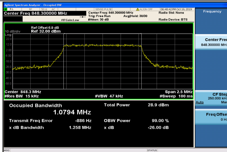
Band5-1.4MHz-16QAM-20643-6RB#0-1.0794
