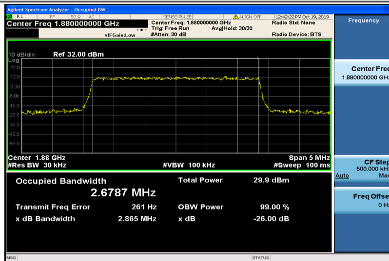
Band2-3MHz-QPSK-18900-15RB#0-2.6787
