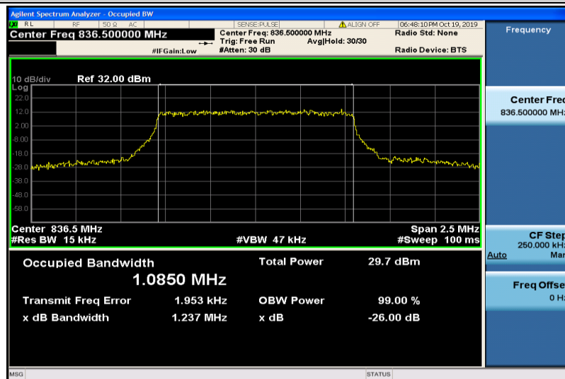
Band5-1.4MHz-QPSK-20525-6RB#0-1.0850
