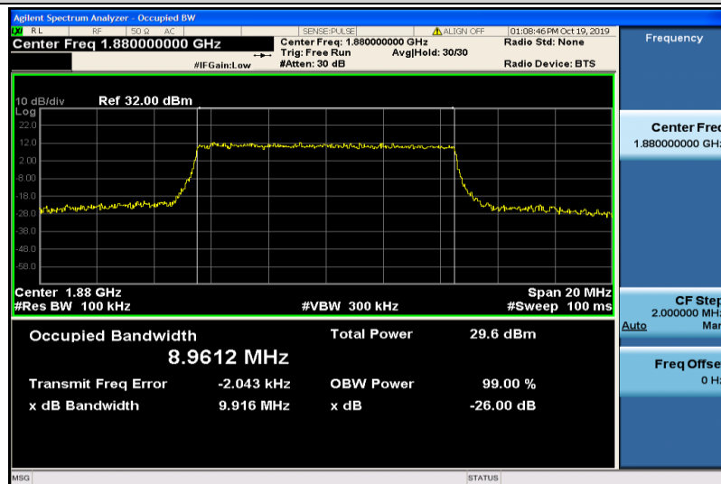
Band2-10MHz-16QAM-18900-50RB#0-8.9612
