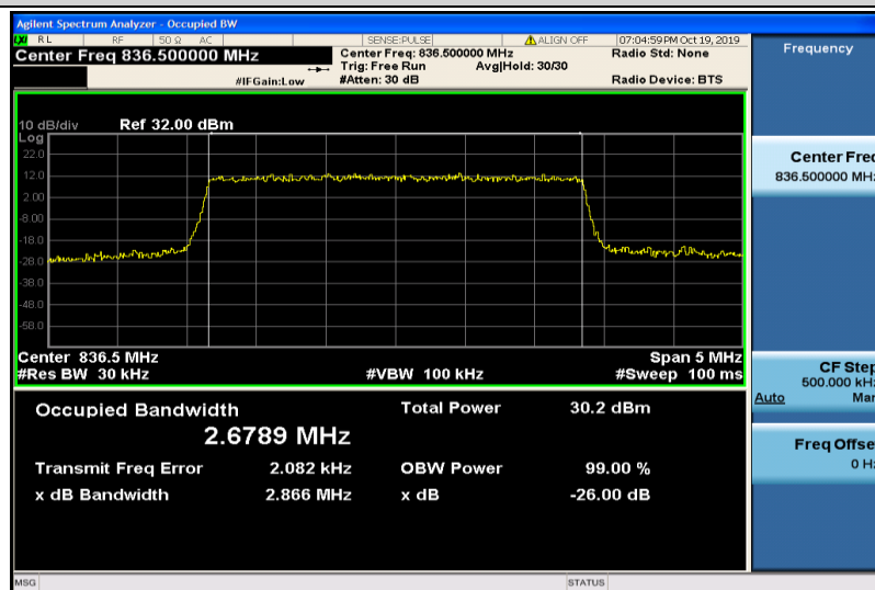
Band5-3MHz-QPSK-20525-15RB#0-2.6789
