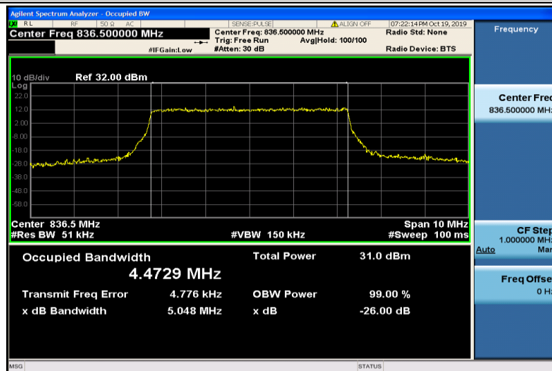
Band5-5MHz-QPSK-20525-25RB#0-4.4729
