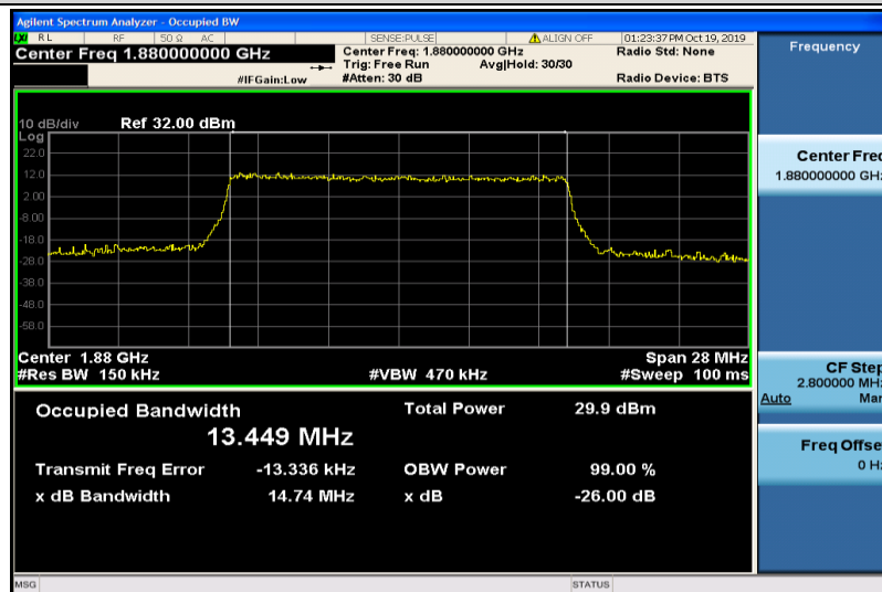
Band2-15MHz-16QAM-18900-75RB#0-13.449
