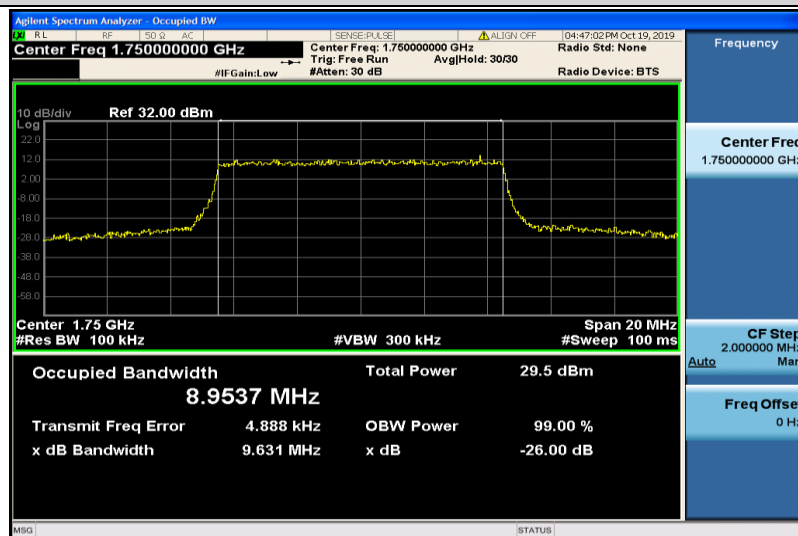
Band4-10MHz-16QAM-20350-50RB#0-8.9537
