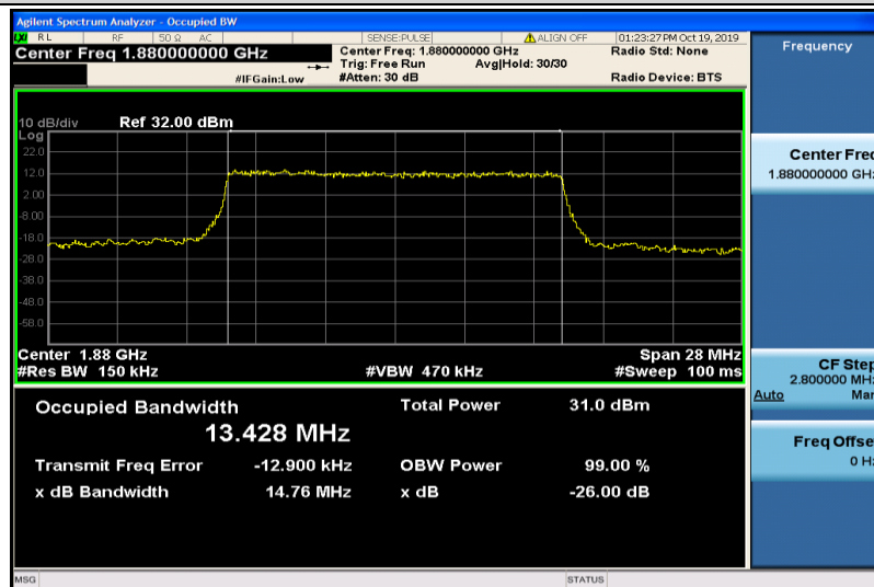
Band2-15MHz-QPSK-18900-75RB#0-13.428
