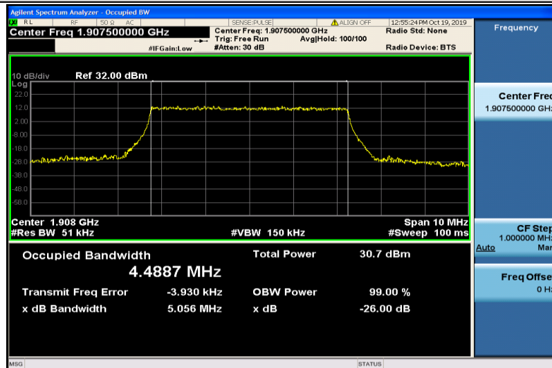
Band2-5MHz-QPSK-19175-25RB#0-4.4887
