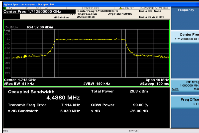
Band4-5MHz-16QAM-19975-25RB#0-4.4860
