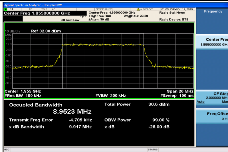
Band2-10MHz-QPSK-18650-50RB#0-8.9523
