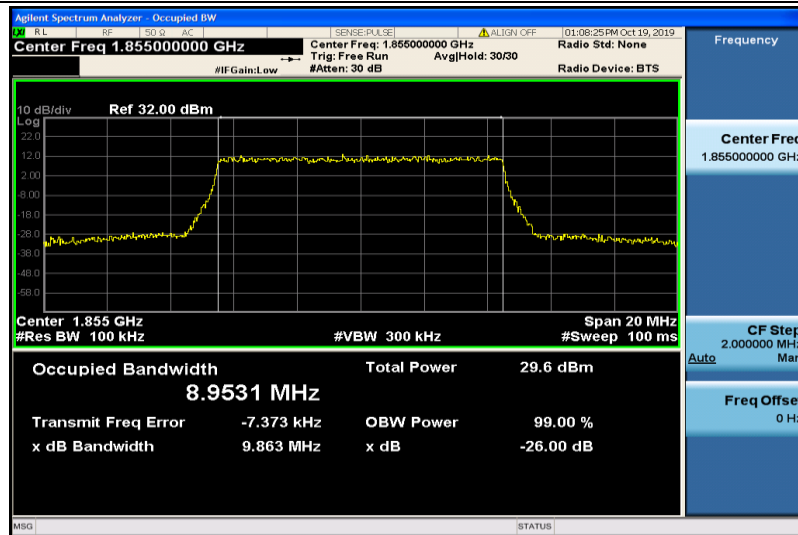
Band2-10MHz-16QAM-18650-50RB#0-8.9531
