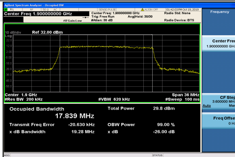
Band2-20MHz-16QAM-19100-100RB#0-17.839
