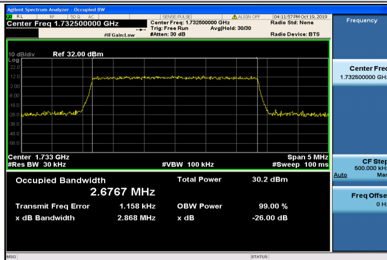
Band4-3MHz-QPSK-20175-15RB#0-2.6767
