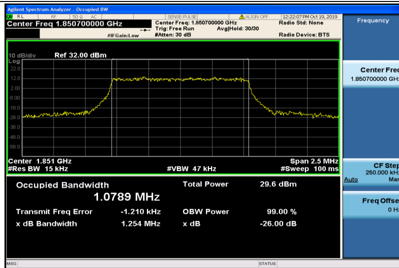
Band2-1.4MHz-QPSK-18607-6RB#0-1.0789
