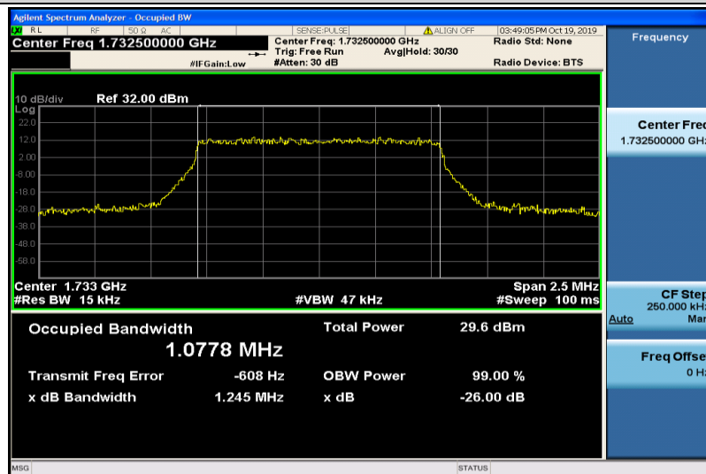
Band4-1.4MHz-QPSK-20175-6RB#0-1.0778
