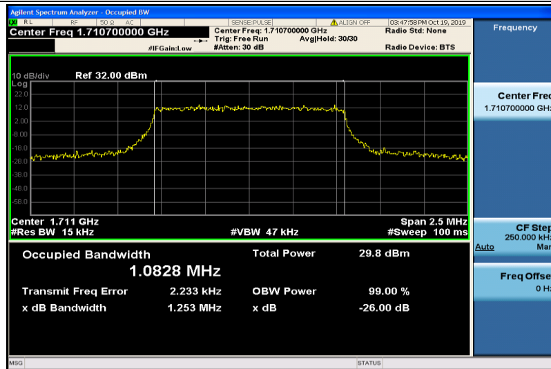
Band4-1.4MHz-QPSK-19957-6RB#0-1.0828
