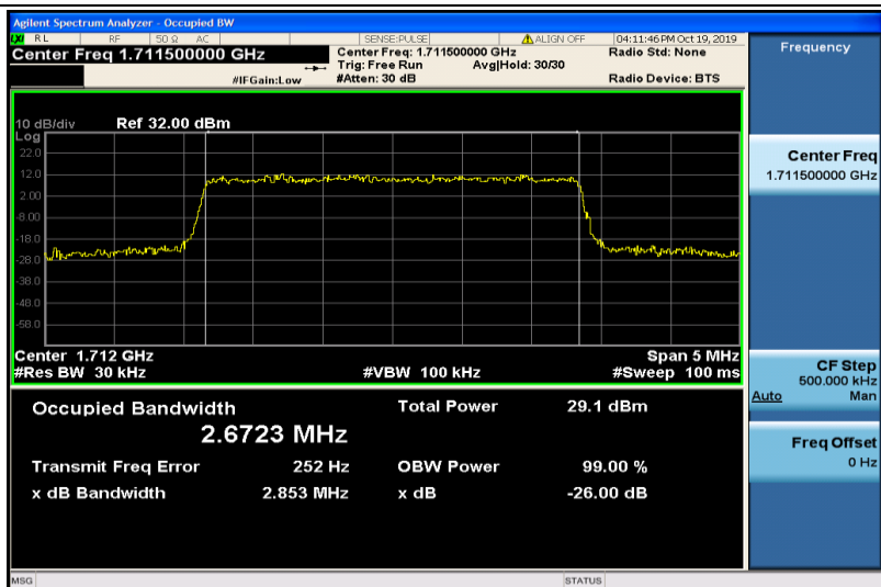
Band4-3MHz-16QAM-19965-15RB#0-2.6723
