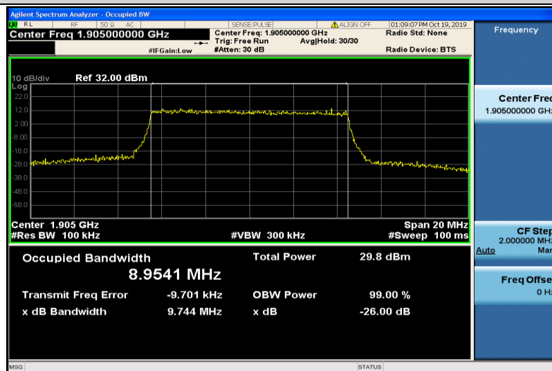
Band2-10MHz-16QAM-19150-50RB#0-8.9541
