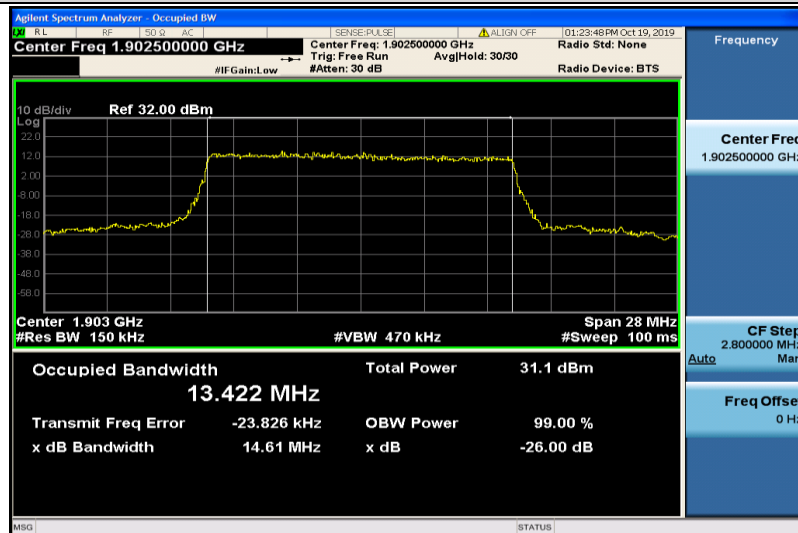
Band2-15MHz-QPSK-19125-75RB#0-13.422
