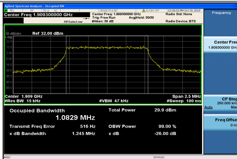
Band2-1.4MHz-QPSK-19193-6RB#0-1.0829
