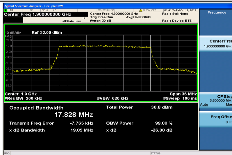
Band2-20MHz-QPSK-19100-100RB#0-17.828
