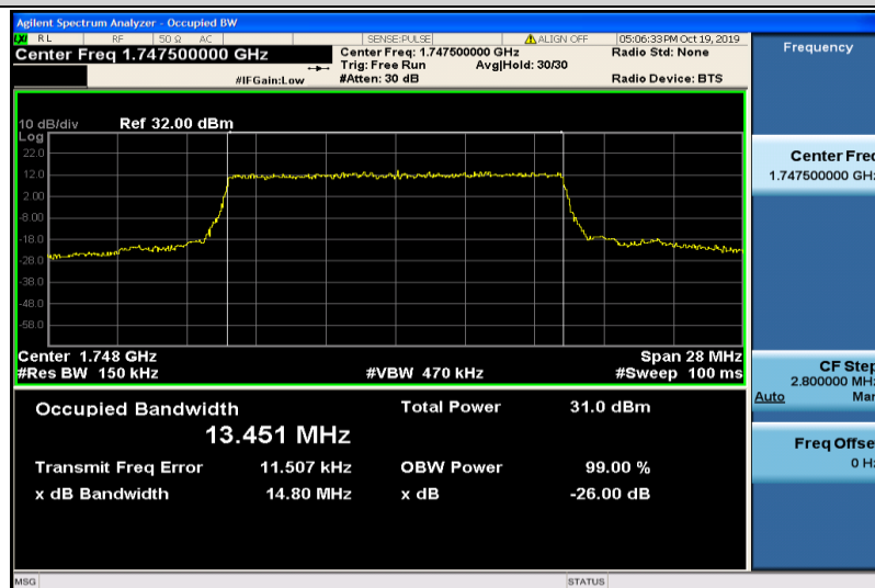
Band4-15MHz-QPSK-20325-75RB#0-13.451
