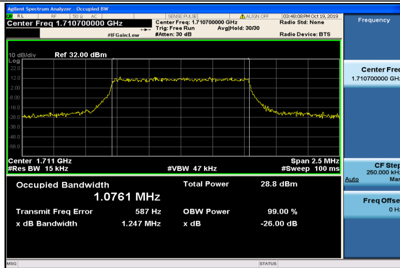
Band4-1.4MHz-16QAM-19957-6RB#0-1.0761
