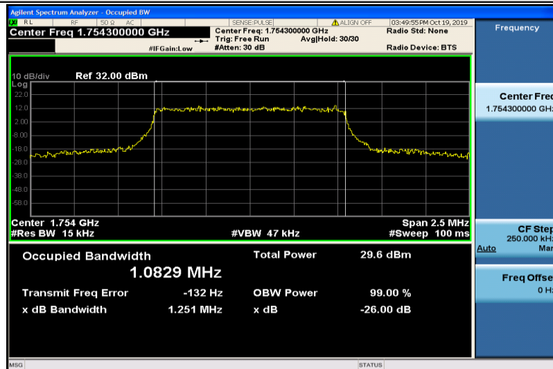
Band4-1.4MHz-QPSK-20393-6RB#0-1.0829
