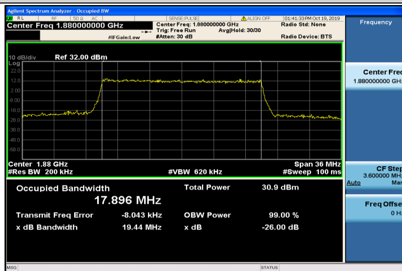
Band2-20MHz-QPSK-18900-100RB#0-17.896
