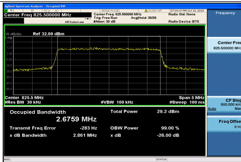
Band5-3MHz-16QAM-20415-15RB#0-2.6759
