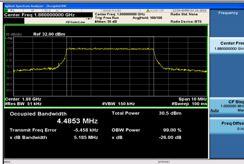
Band2-5MHz-QPSK-18900-25RB#0-4.4853
