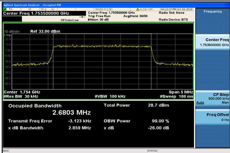
Band4-3MHz-16QAM-20385-15RB#0-2.6803
