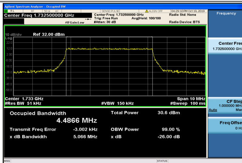
Band4-5MHz-QPSK-20175-25RB#0-4.4866
