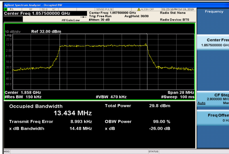
Band2-15MHz-16QAM-18675-75RB#0-13.434
