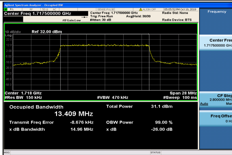
Band4-15MHz-QPSK-20025-75RB#0-13.409
