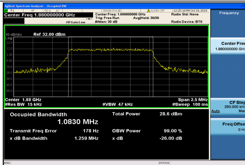
Band2-1.4MHz-16QAM-18900-6RB#0-1.0830
