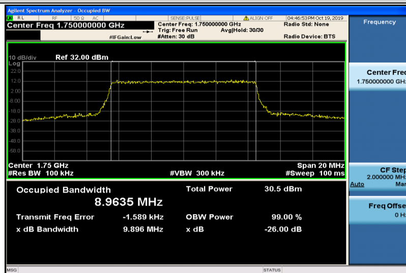
Band4-10MHz-QPSK-20350-50RB#0-8.9635
