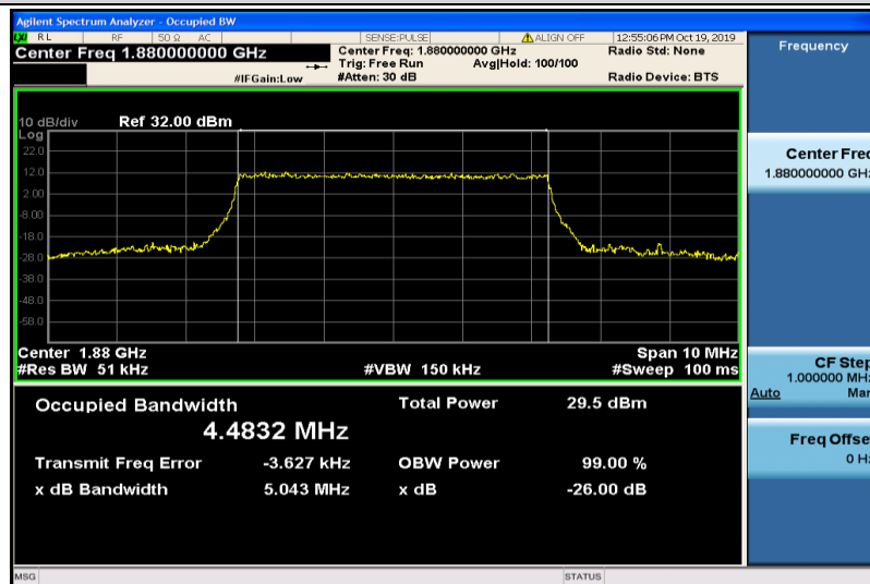
Band2-5MHz-16QAM-18900-25RB#0-4.4832
