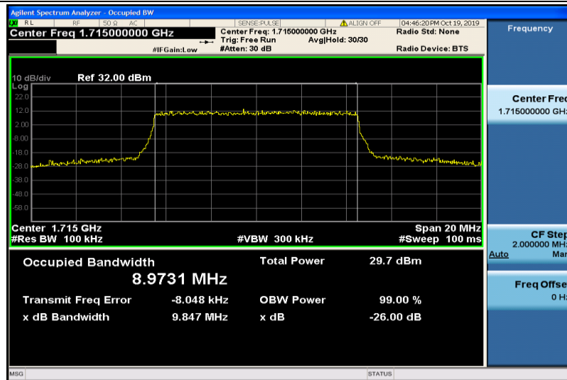
Band4-10MHz-16QAM-20000-50RB#0-8.9731
