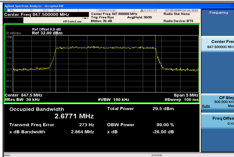
Band5-3MHz-16QAM-20635-15RB#0-2.6771
