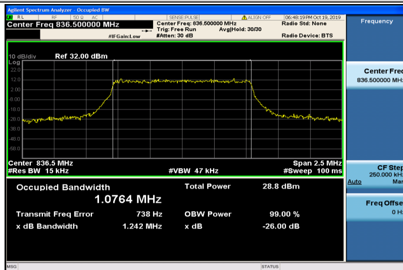
Band5-1.4MHz-16QAM-20525-6RB#0-1.0764
