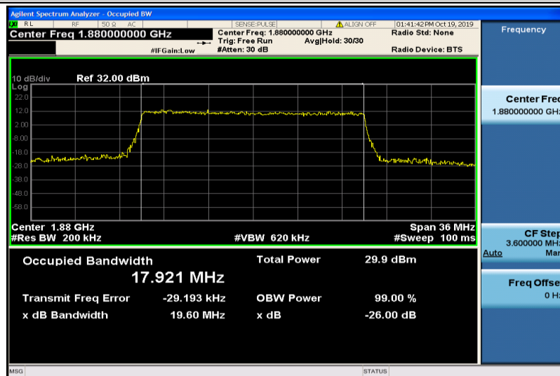
Band2-20MHz-16QAM-18900-100RB#0-17.921
