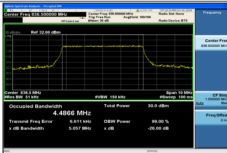
Band5-5MHz-16QAM-20525-25RB#0-4.4866
