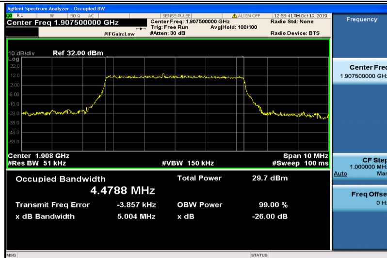
Band2-5MHz-16QAM-19175-25RB#0-4.4788
