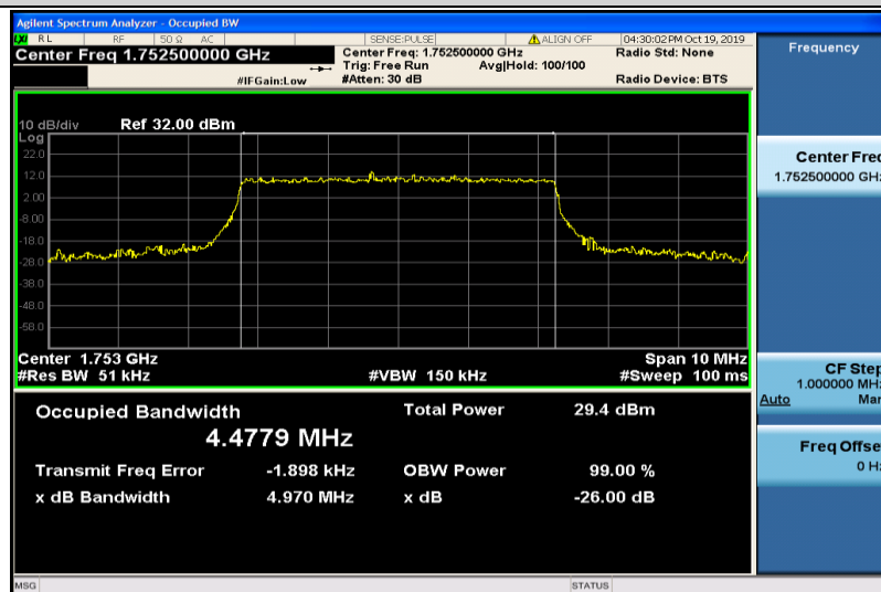
Band4-5MHz-16QAM-20375-25RB#0-4.4779
