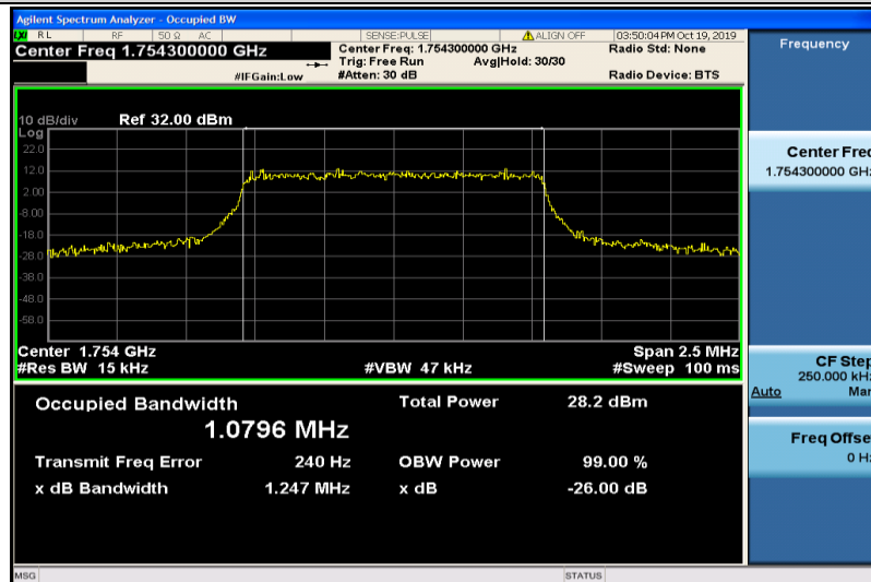
Band4-1.4MHz-16QAM-20393-6RB#0-1.0796
