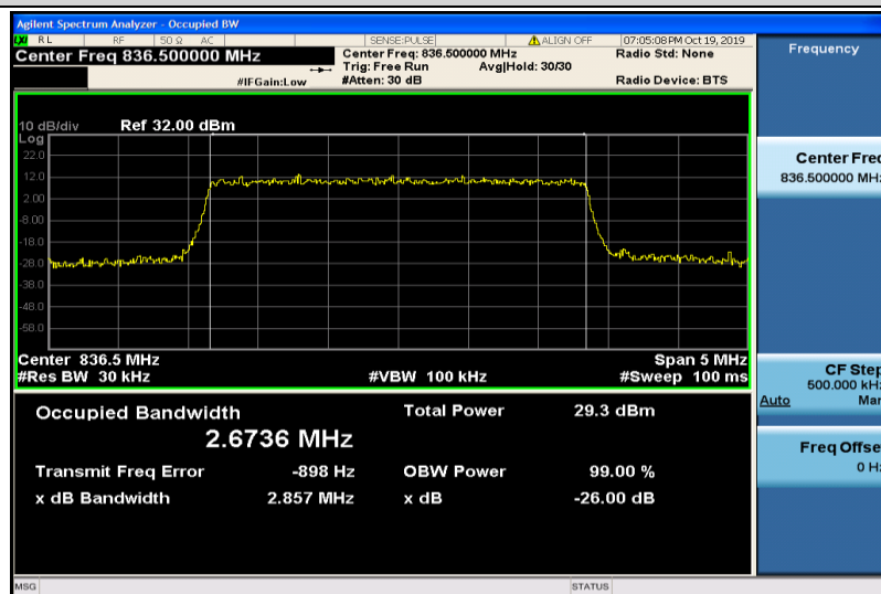
Band5-3MHz-16QAM-20525-15RB#0-2.6736
