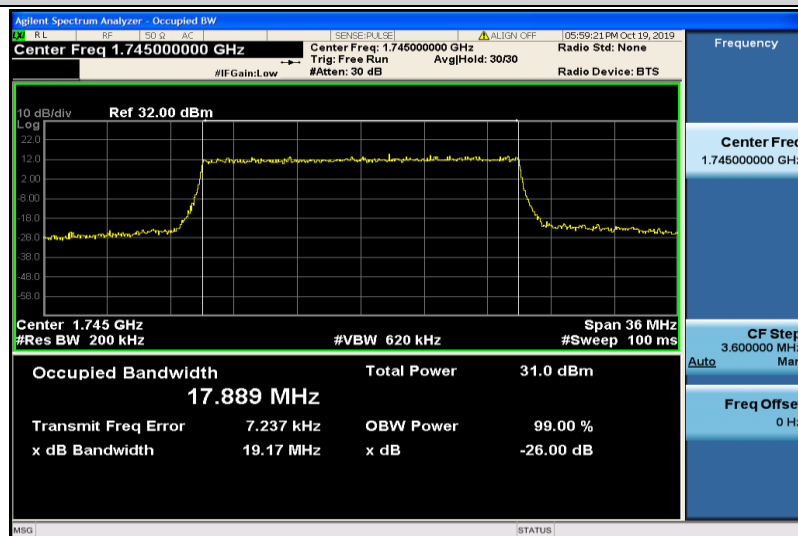
Band4-20MHz-QPSK-20300-100RB#0-17.889
