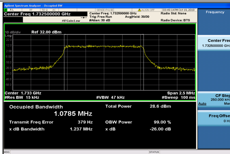
Band4-1.4MHz-16QAM-20175-6RB#0-1.0785
