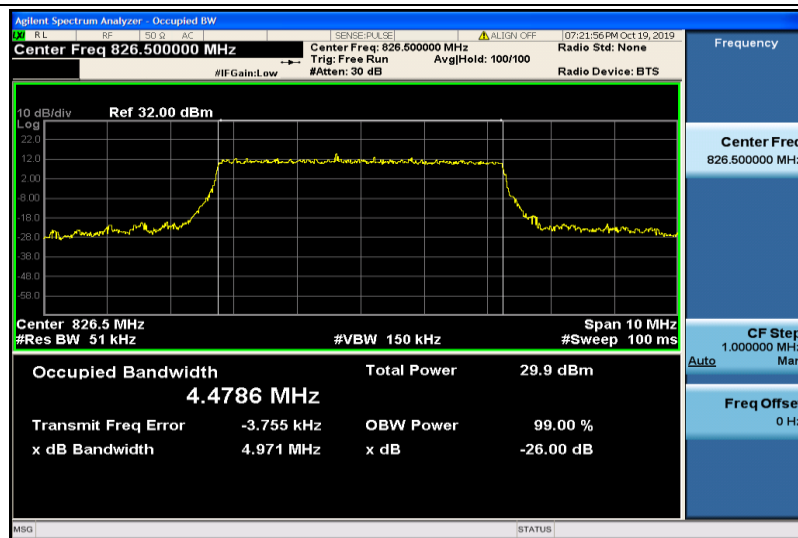
Band5-5MHz-16QAM-20425-25RB#0-4.4786
