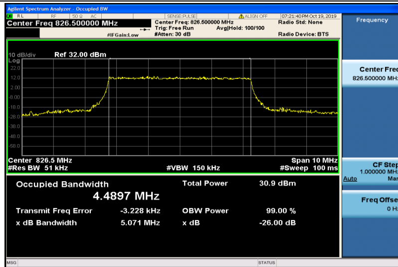
Band5-5MHz-QPSK-20425-25RB#0-4.4897
