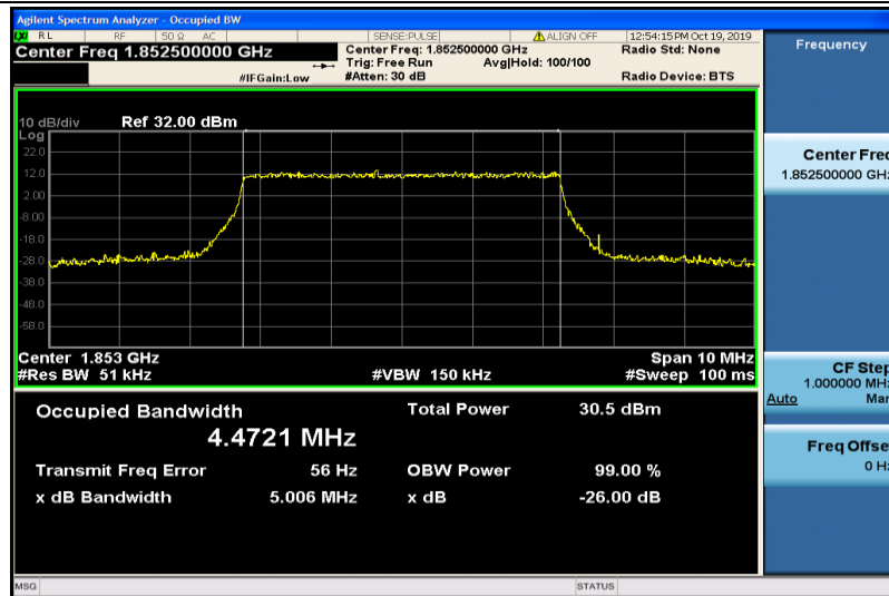
Band2-5MHz-QPSK-18625-25RB#0-4.4721
