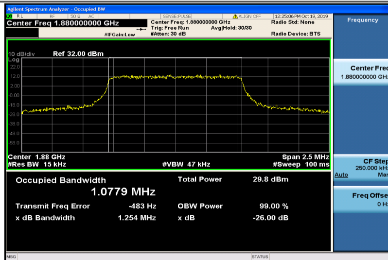
Band2-1.4MHz-QPSK-18900-6RB#0-1.0779
