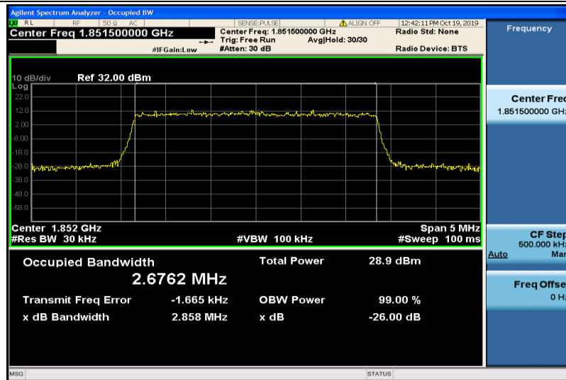
Band2-3MHz-16QAM-18615-15RB#0-2.6762
