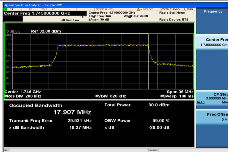
Band4-20MHz-16QAM-20300-100RB#0-17.907
