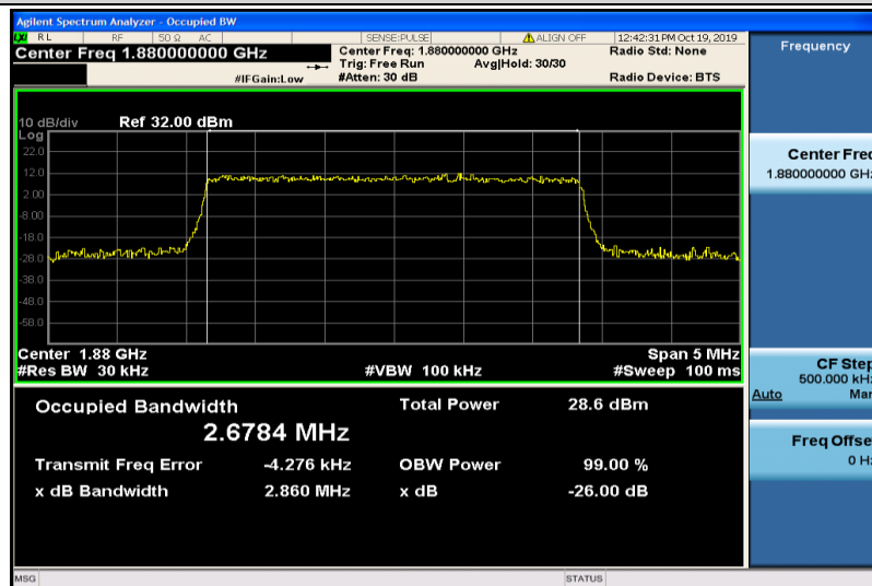
Band2-3MHz-16QAM-18900-15RB#0-2.6784
