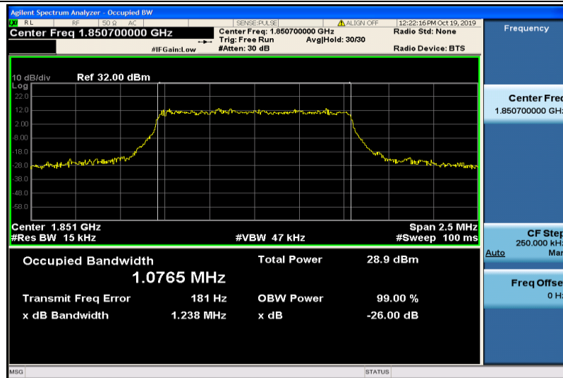
Band2-1.4MHz-16QAM-18607-6RB#0-1.0765
