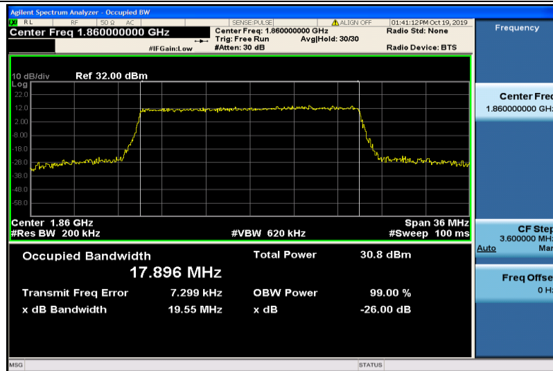
Band2-20MHz-QPSK-18700-100RB#0-17.896
