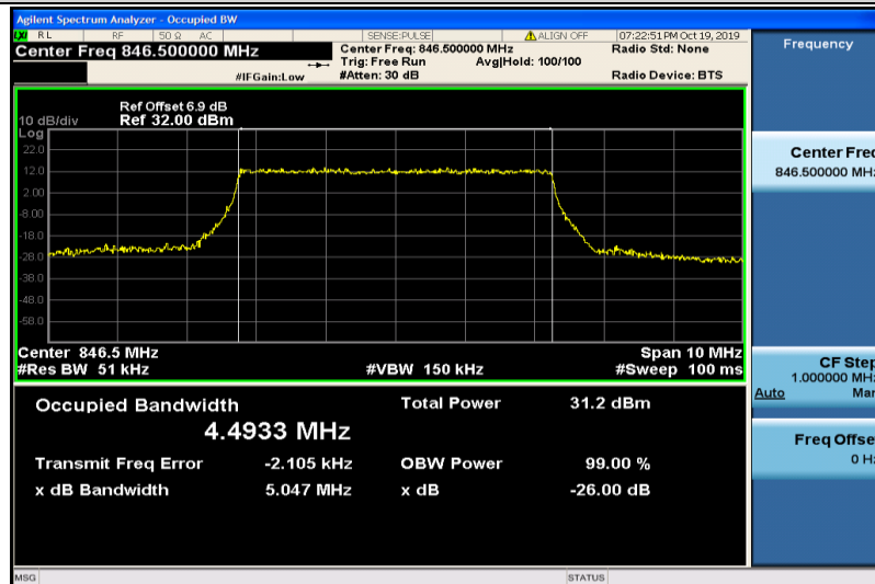
Band5-5MHz-QPSK-20625-25RB#0-4.4933
