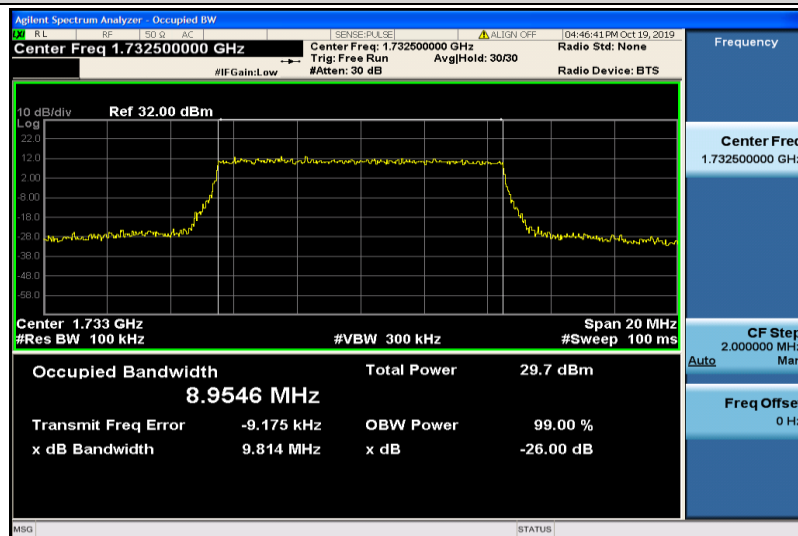
Band4-10MHz-16QAM-20175-50RB#0-8.9546
