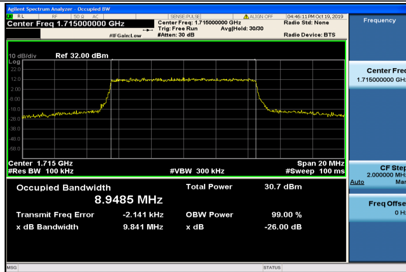
Band4-10MHz-QPSK-20000-50RB#0-8.9485
