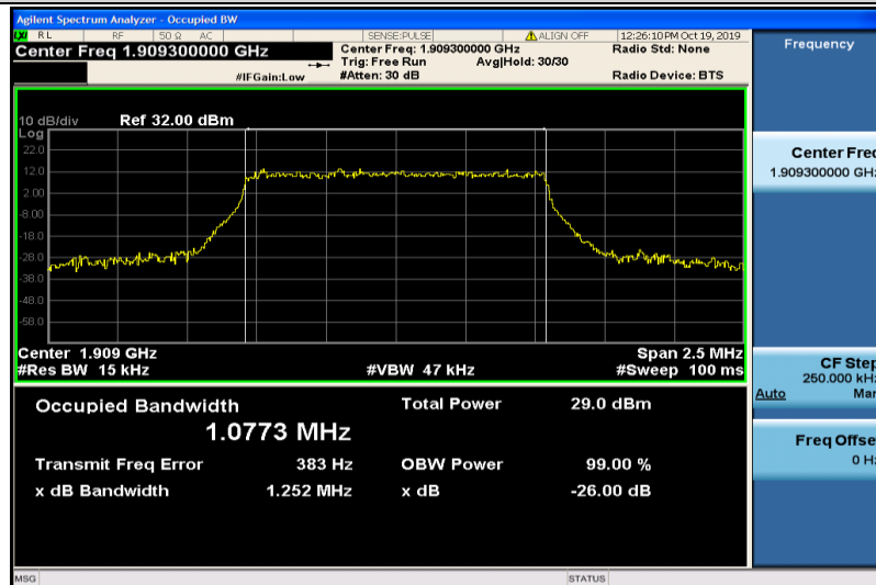
Band2-1.4MHz-16QAM-19193-6RB#0-1.0773
