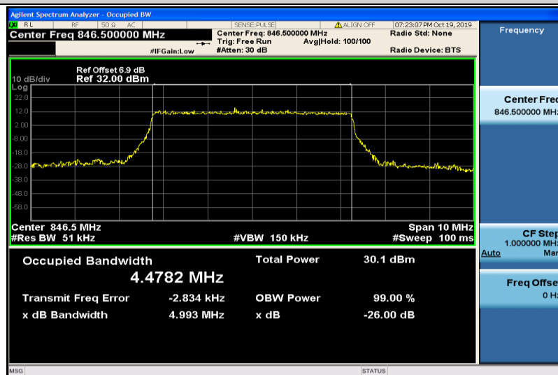
Band5-5MHz-16QAM-20625-25RB#0-4.4782
