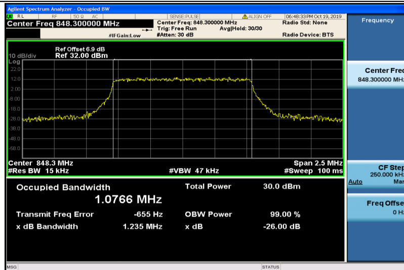
Band5-1.4MHz-QPSK-20643-6RB#0-1.0766
