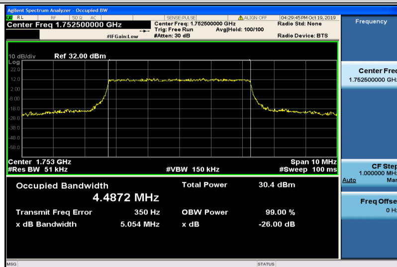
Band4-5MHz-QPSK-20375-25RB#0-4.4872
