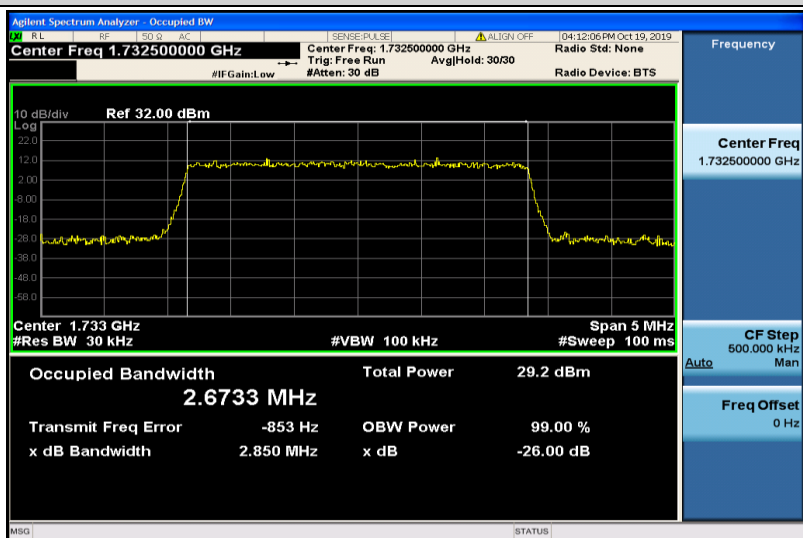
Band4-3MHz-16QAM-20175-15RB#0-2.6733
