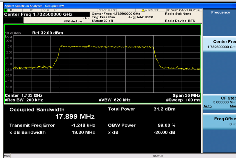
Band4-20MHz-QPSK-20175-100RB#0-17.899
