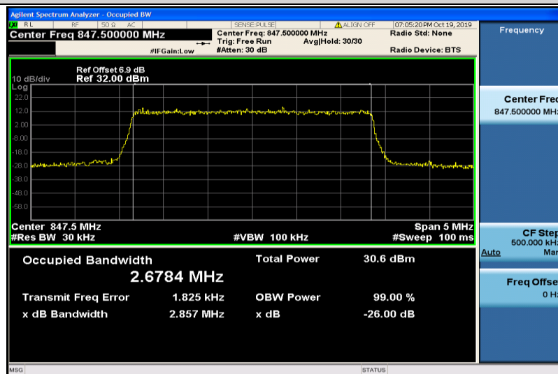
Band5-3MHz-QPSK-20635-15RB#0-2.6784
