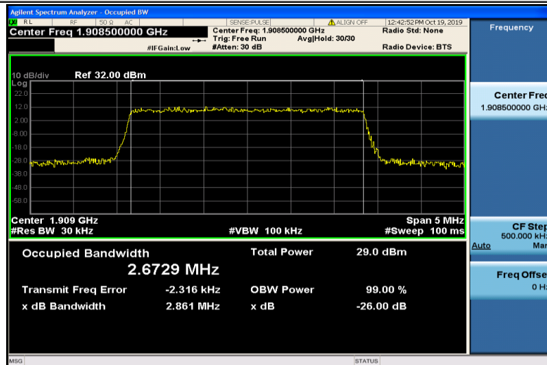
Band2-3MHz-16QAM-19185-15RB#0-2.6729
