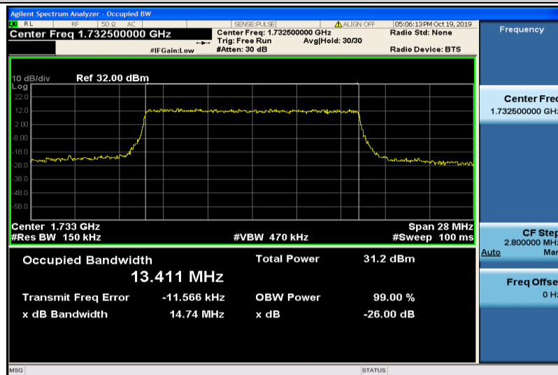
Band4-15MHz-QPSK-20175-75RB#0-13.411
