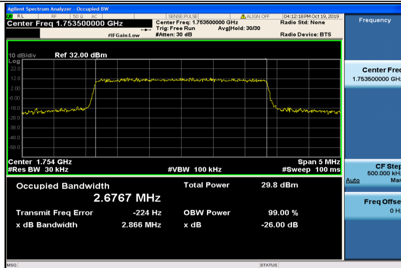
Band4-3MHz-QPSK-20385-15RB#0-2.6767
