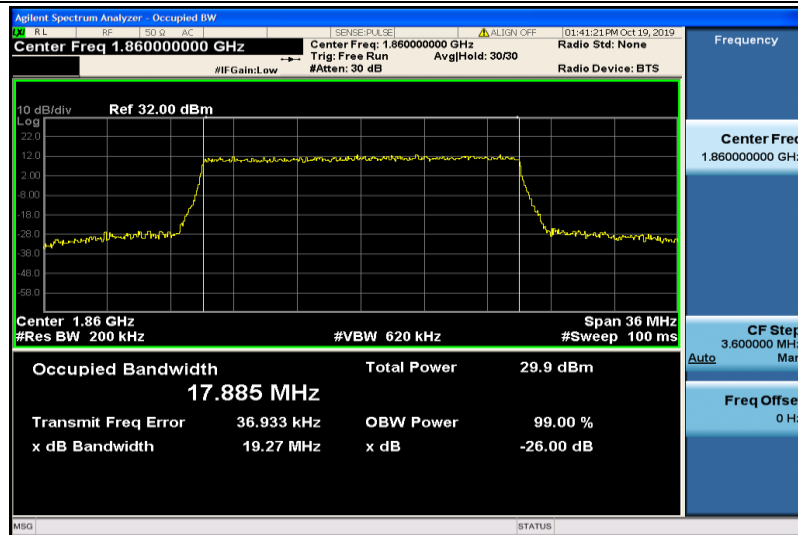
Band2-20MHz-16QAM-18700-100RB#0-17.885
