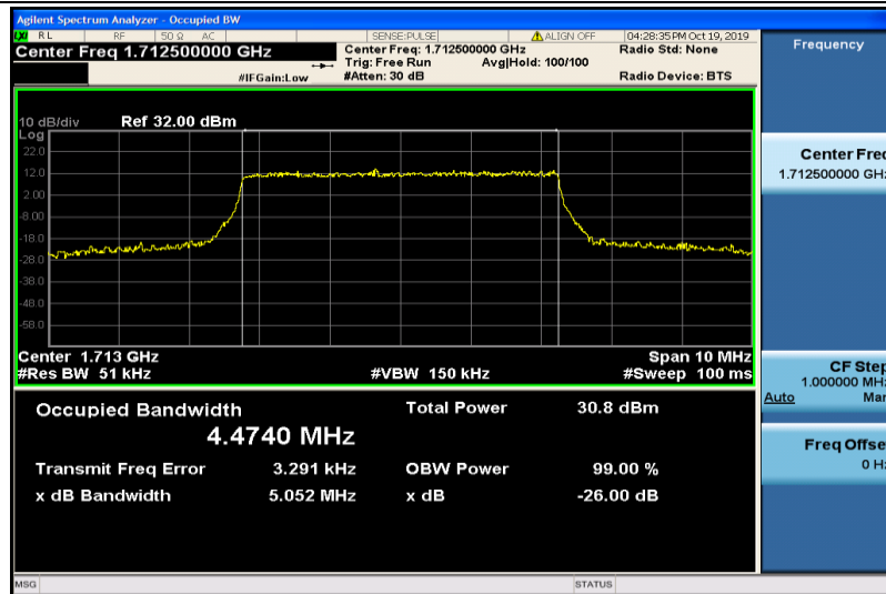
Band4-5MHz-QPSK-19975-25RB#0-4.4740
