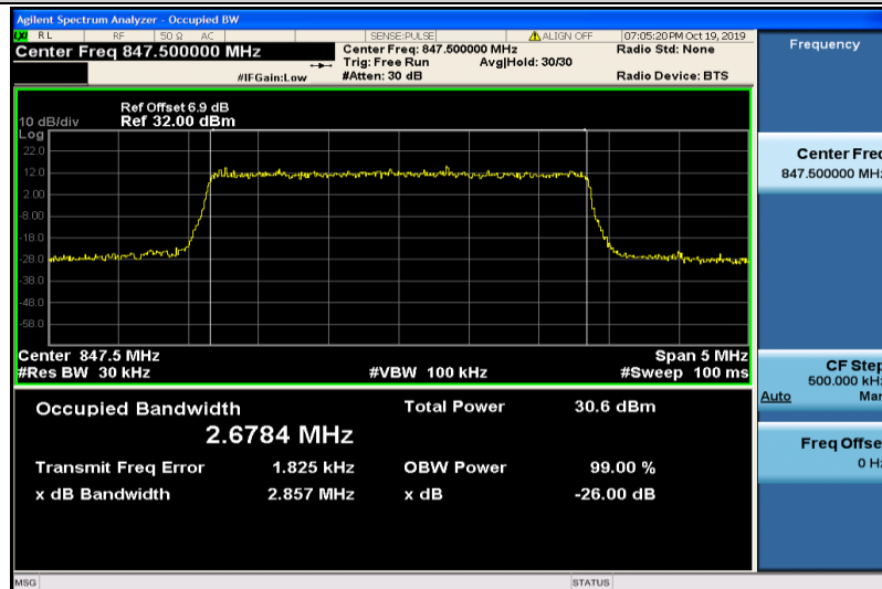
Band5-3MHz-QPSK-20635-15RB#0-2.6784
