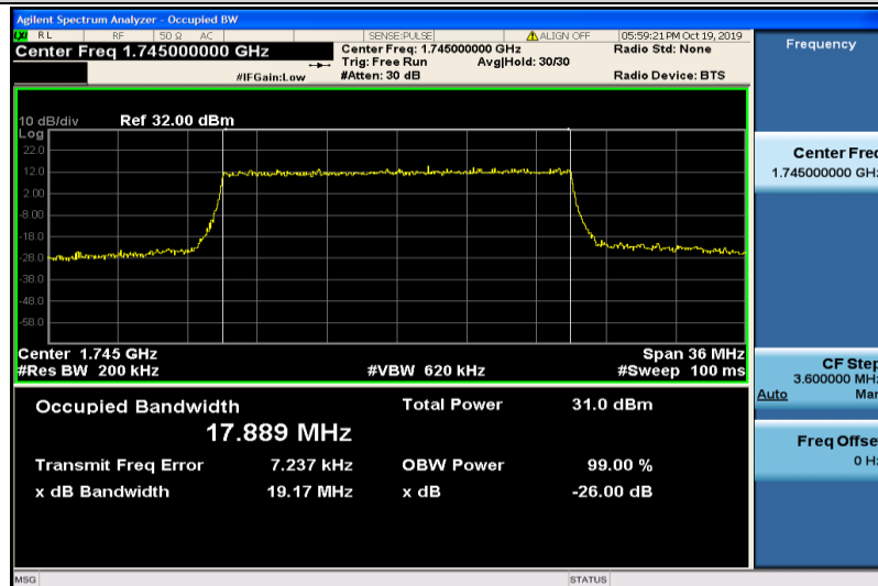
Band4-20MHz-QPSK-20300-100RB#0-17.889
