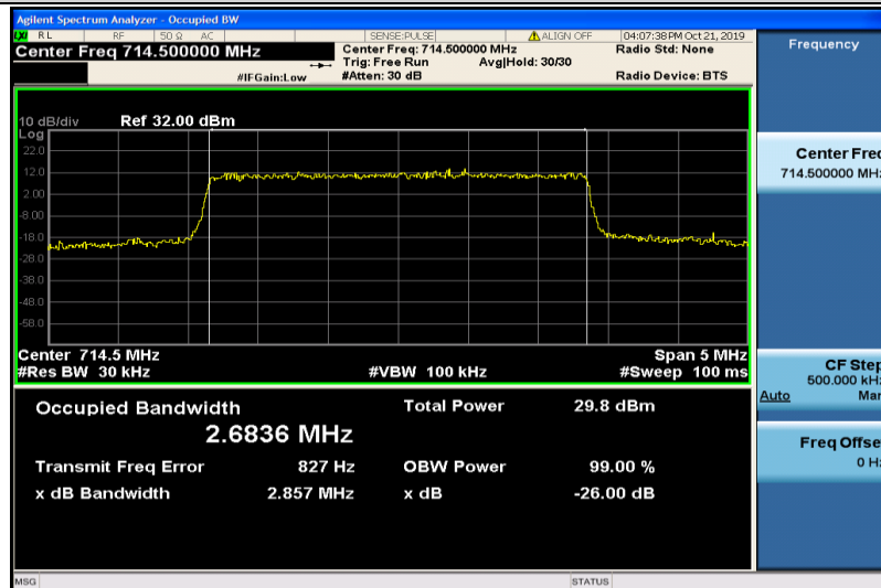
Band12-3MHz-16QAM-23165-15RB#0-2.6836
