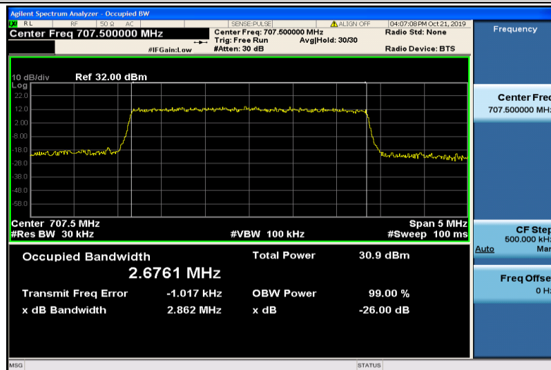
Band12-3MHz-QPSK-23095-15RB#0-2.6761
