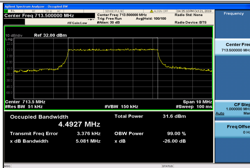
Band12-5MHz-QPSK-23155-25RB#0-4.4927
