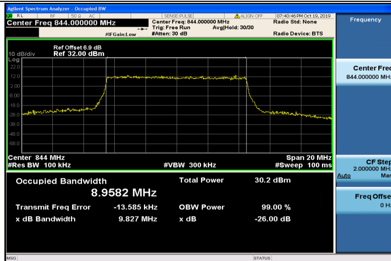
Band5-10MHz-16QAM-20600-50RB#0-8.9582
