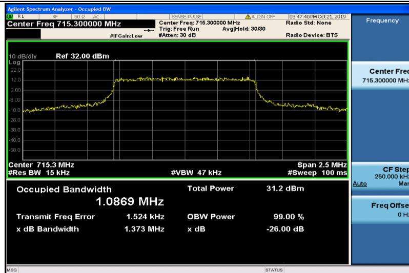
Band12-1.4MHz-QPSK-23173-6RB#0-1.0869
