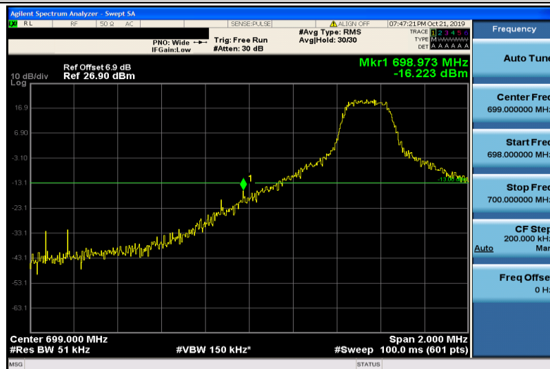
Band12-5MHz-QPSK-23035-1RB#0
