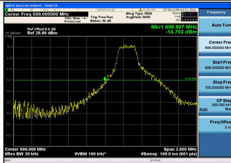
Band12-3MHz-16QAM-23025-1RB#0
