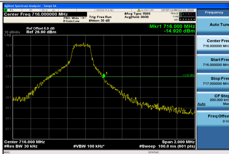
Band12-3MHz-16QAM-23165-1RB#14
