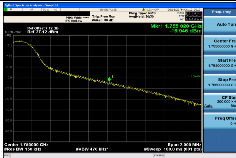
Band4-15MHz-16QAM-20325-1RB#74
