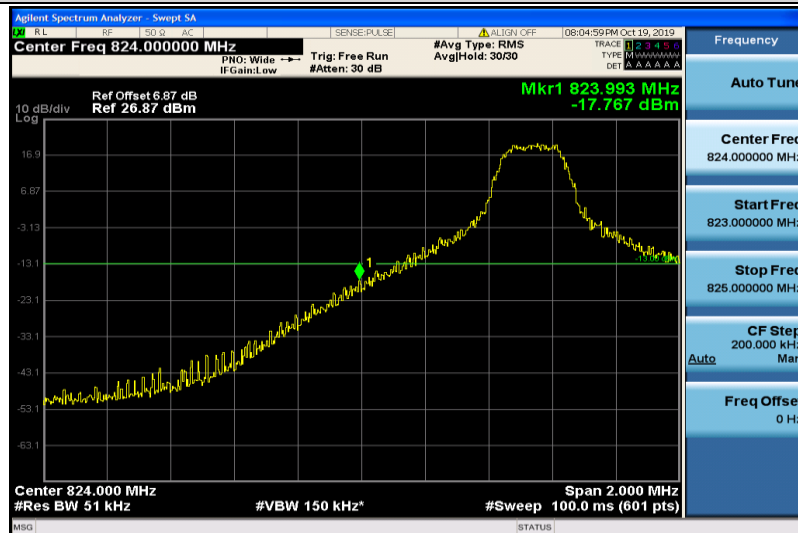
Band5-5MHz-QPSK-20425-1RB#0
