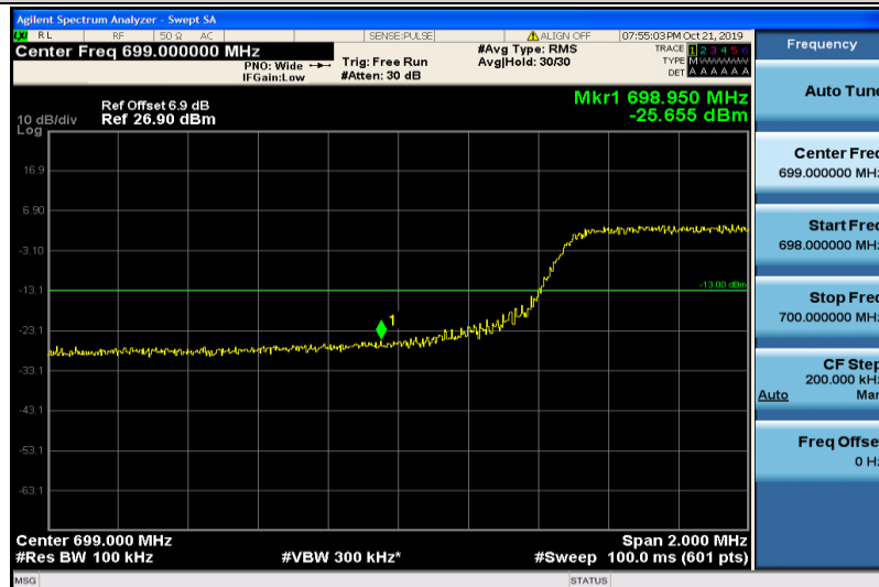
Band12-10MHz-16QAM-23060-50RB#0
