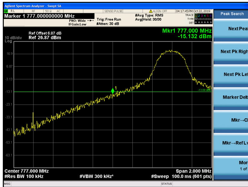
Band13-10MHz-16QAM-23230-1RB#0
