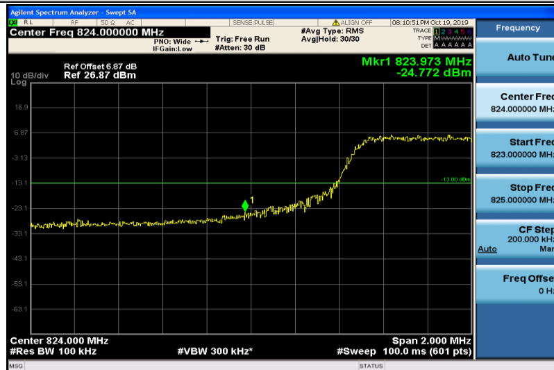
Band5-10MHz-QPSK-20450-50RB#0
