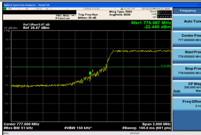
Band13-5MHz-16QAM-23205-25RB#0
