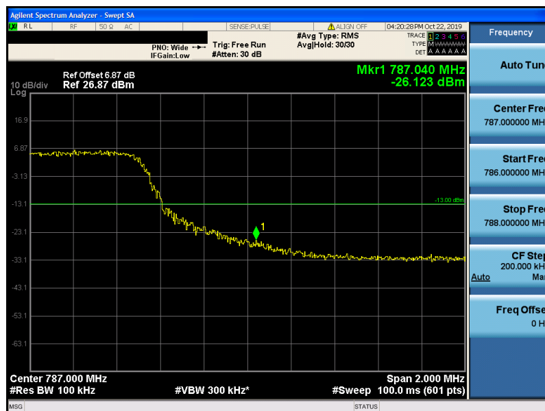
Band13-10MHz-QPSK-23230-50RB#0
