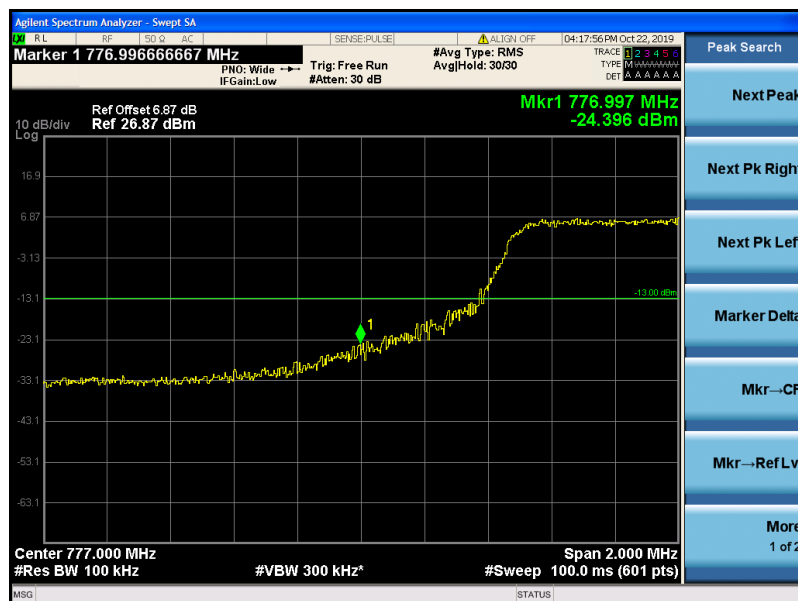
Band13-10MHz-QPSK-23230-50RB#0
