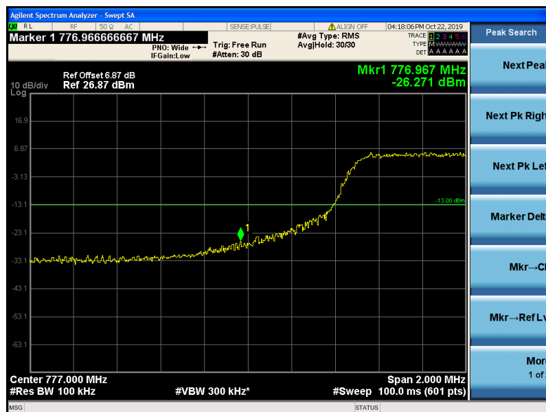
Band13-10MHz-16QAM-23230-50RB#0
