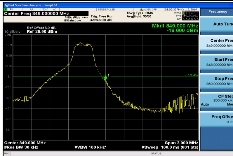
Band5-3MHz-16QAM-20635-1RB#14
