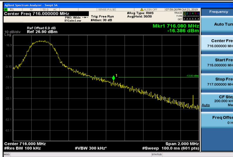
Band12-10MHz-16QAM-23130-1RB#49
