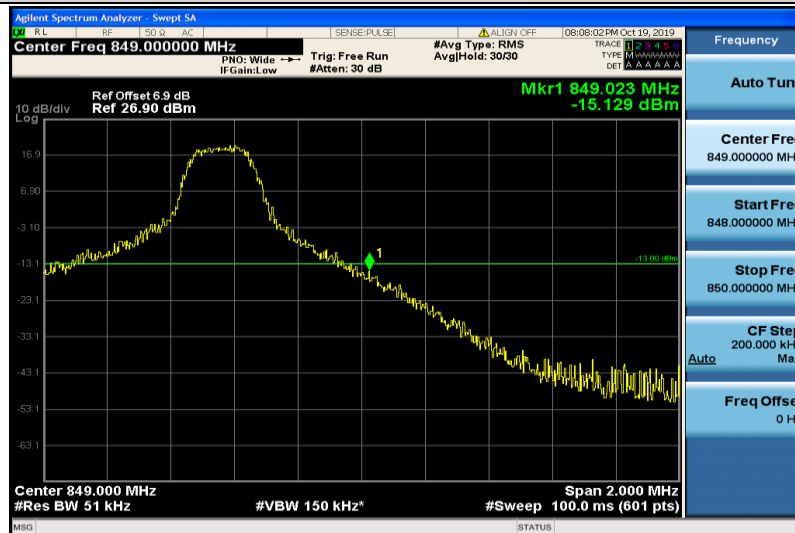
Band5-5MHz-16QAM-20625-1RB#24
