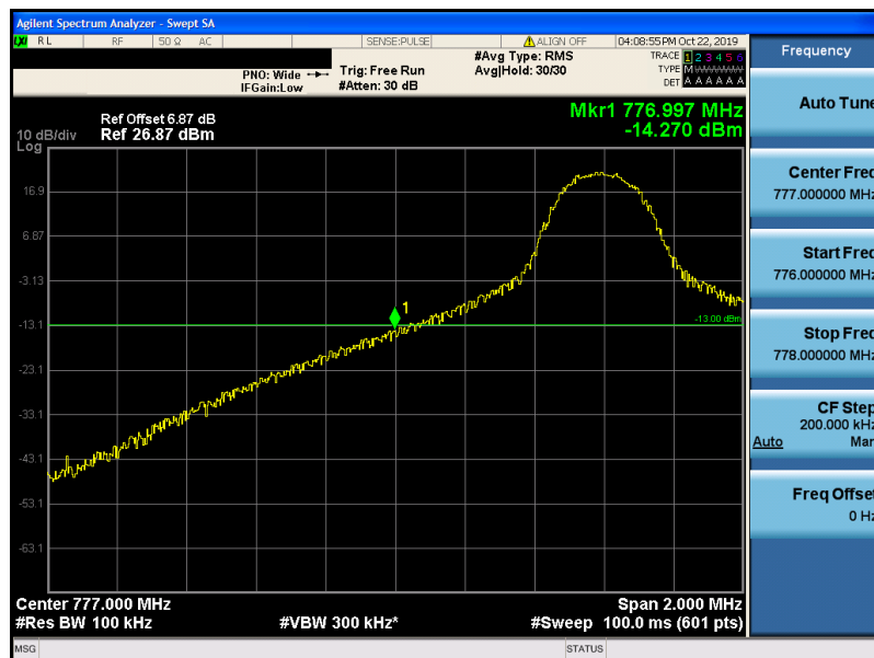
Band13-10MHz-QPSK-23230-1RB#0
