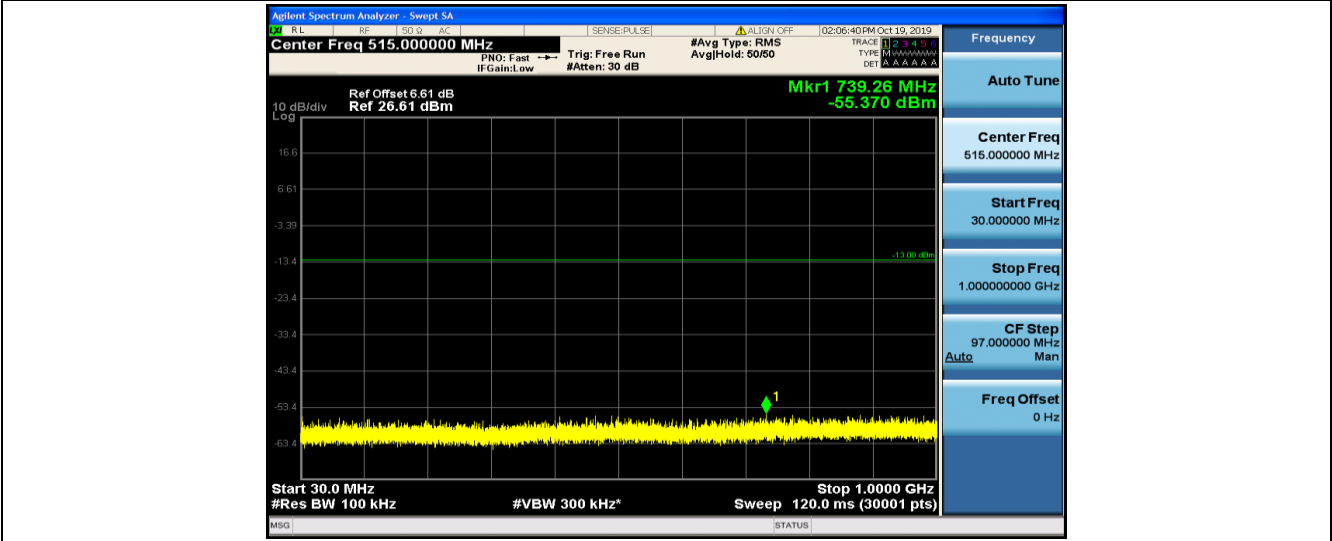
Band2-1.4MHz-QPSK-19193-1RB#0-30~1000MHz
