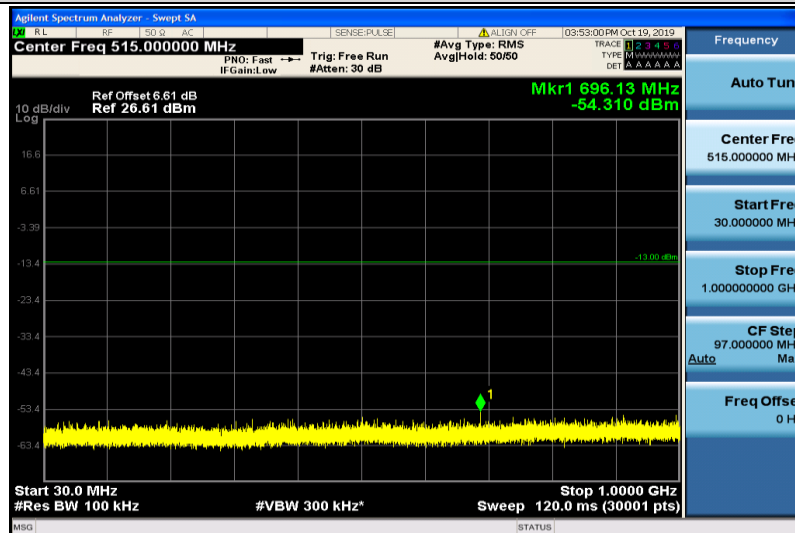
Band4-1.4MHz-QPSK-20175-1RB#0-30~1000MHz
