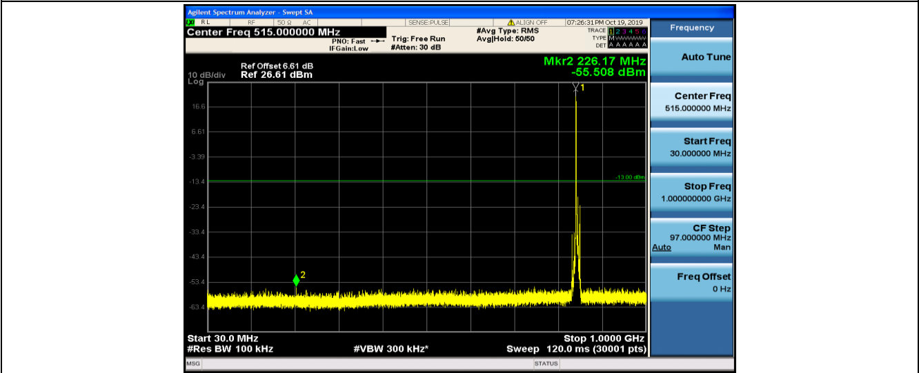
Band5-5MHz-16QAM-20625-1RB#0-30~1000MHz
