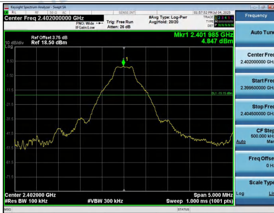
2_Bandedge_NVNT_ANT1_1-DH5_2402_00
