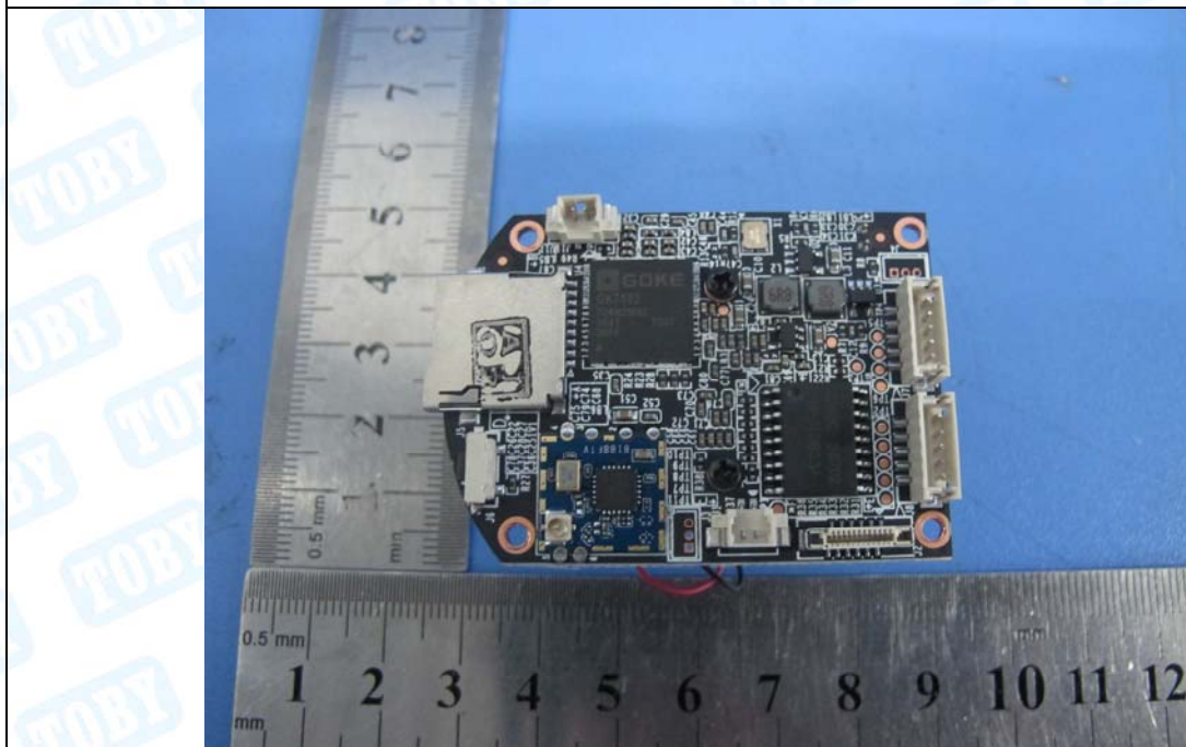
Photo 17 Internal of PCB
