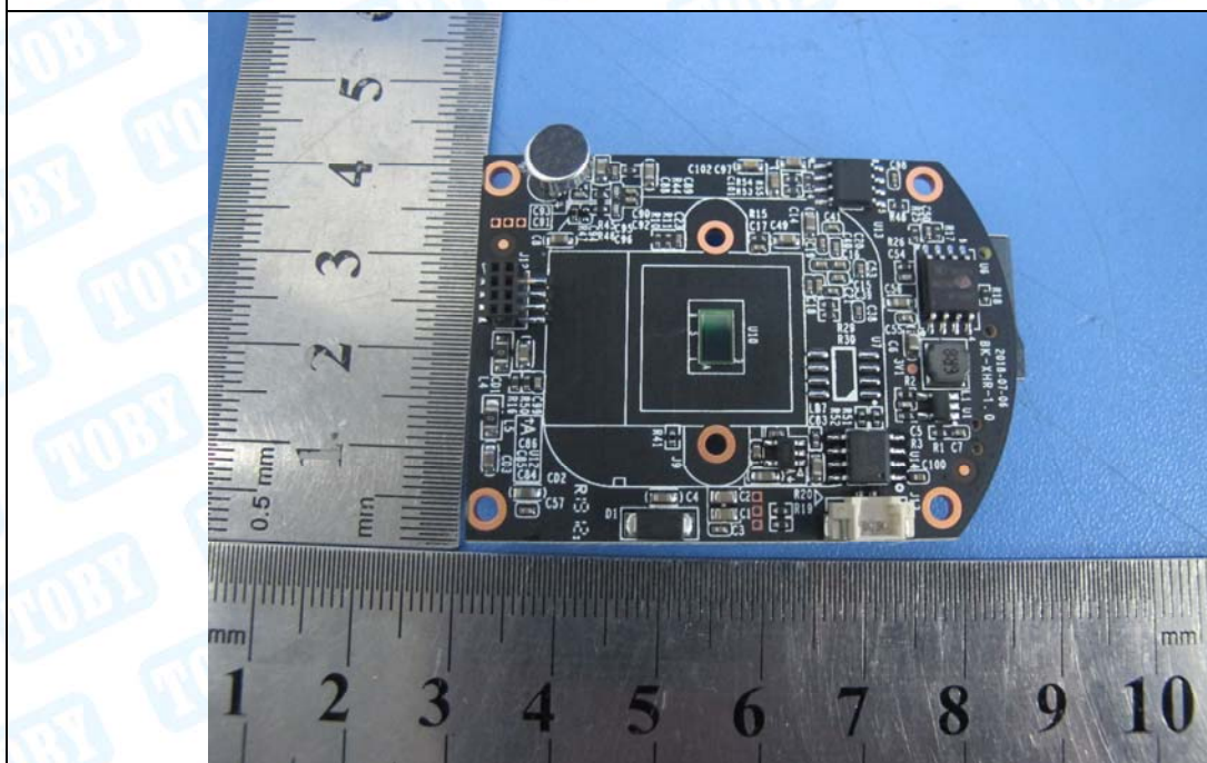
Photo 15 Internal of PCB
