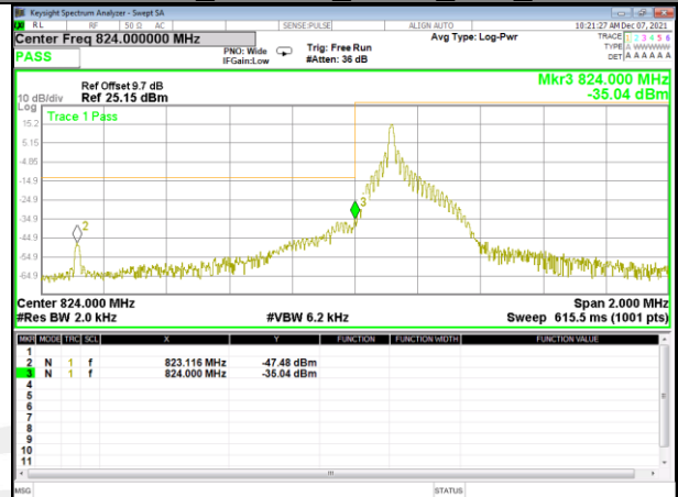
Band5_3.75kHz_QPSK_Low_1#0
