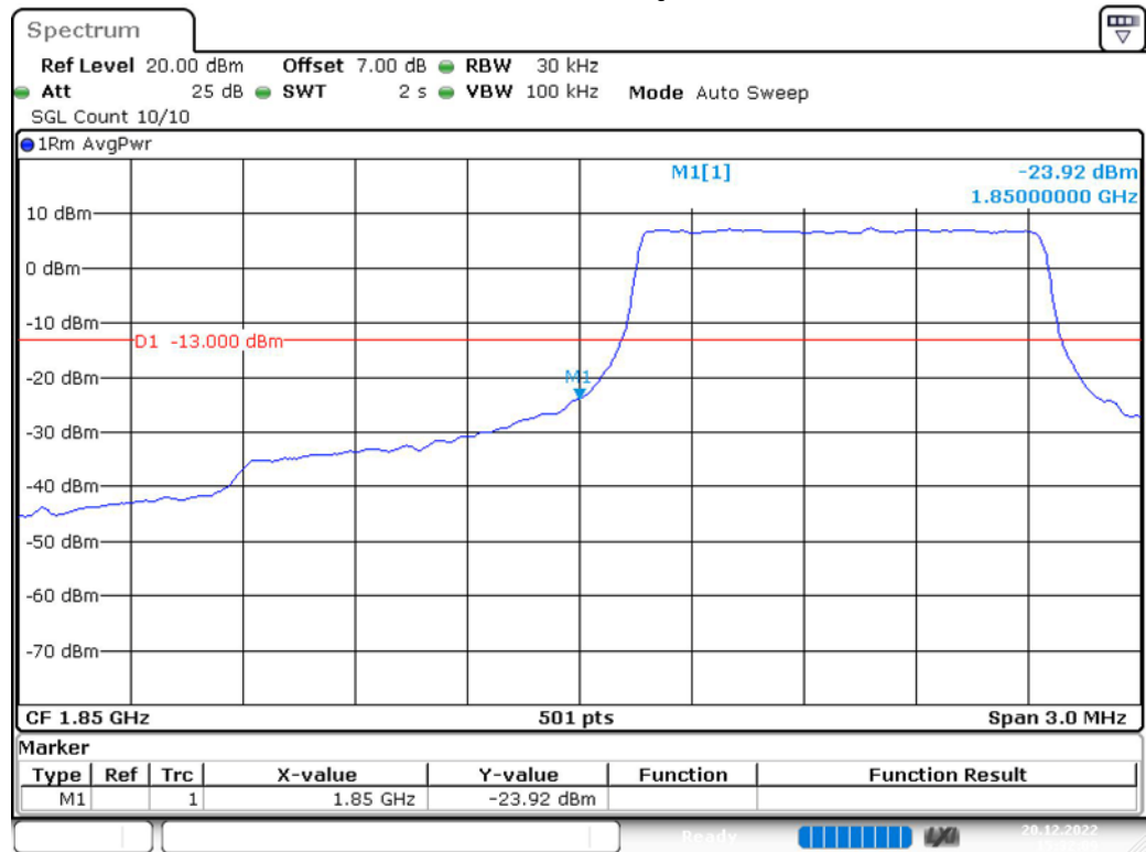
Band 2_1.4 MHz_Low_QPSK_RB6#0
