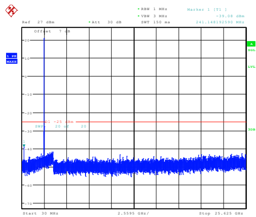
15MHz_High_QPSK_1@0 -39.08dBm
