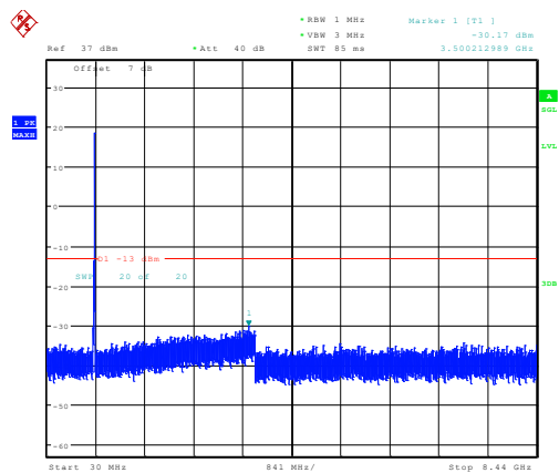
10MHz_High_QPSK_50@0 -30.17dBm
