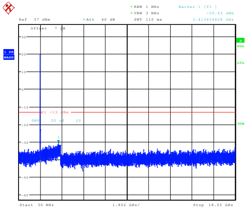
10MHz_Low_QPSK_1@0 -30.43dBm
