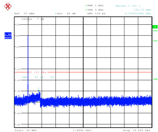
15MHz_High_QPSK_75@0 -30.73dBm
