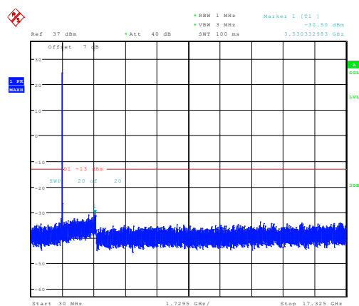
15MHz_Middle_QPSK_1@0 -30.50dBm
