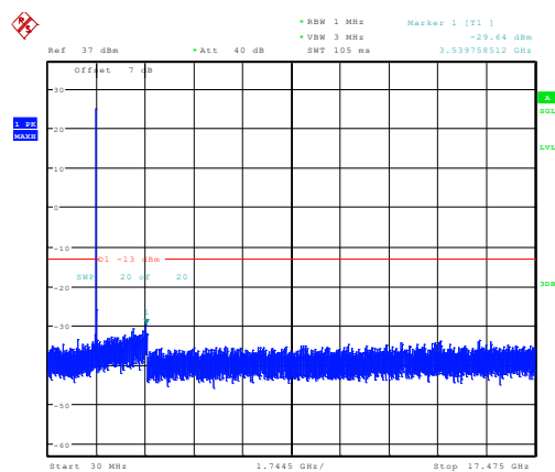
15MHz_High_QPSK_1@0 -29.64dBm
