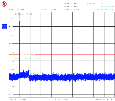
1.4MHz_Middle_QPSK_6@0 -30.99dBm
