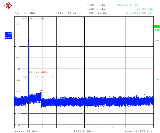
15MHz_Low_QPSK_75@0 -30.83dBm
