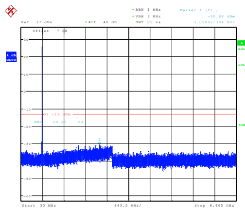
5MHz_High_QPSK_1@0 -30.88dBm
