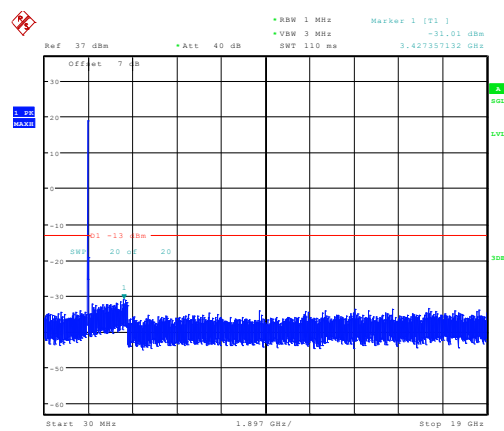
20MHz_High_QPSK_100@0 -31.01dBm
