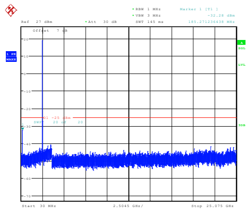
15MHz_Low_QPSK_1@0 -32.28dBm
