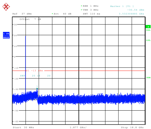
3MHz_Middle_QPSK_15@0 -30.54dBm
