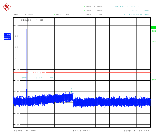
3MHz_Low_QPSK_1@0 -31.15dBm
