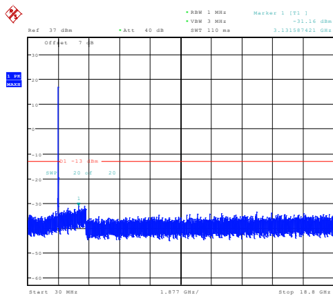
15MHz_Middle_QPSK_1@0 -31.16dBm
