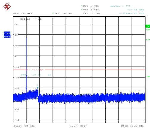
20MHz_Middle_QPSK_100@0 -30.58dBm
