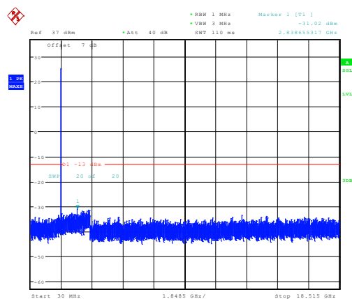
3MHz_Low_QPSK_1@0 -31.02dBm
