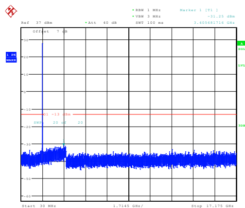
15MHz_Low_QPSK_1@0 -31.25dBm
