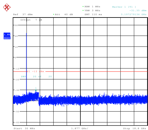
5MHz_Middle_QPSK_1@0 -31.35dBm
