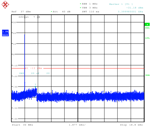
10MHz_Middle_QPSK_1@0 -31.18dBm
