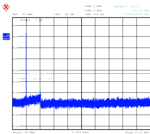
10MHz_High_QPSK_1@0 -31.02dBm
