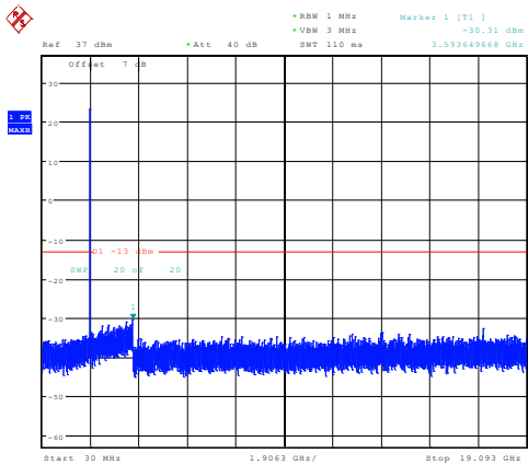
1.4MHz_High_QPSK_6@0 -30.31dBm
