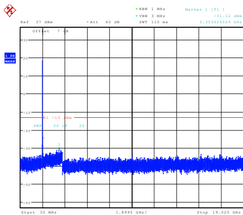
15MHz_High_QPSK_1@0 -31.12dBm
