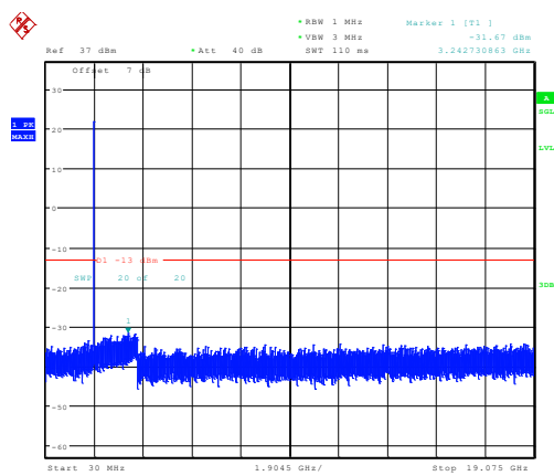
5MHz_High_QPSK_25@0 -31.67dBm
