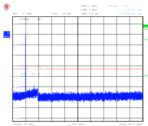
20MHz_Low_QPSK_1@0 -30.82dBm
