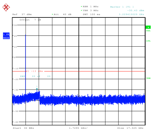
5MHz_Middle_QPSK_25@0 -30.43dBm
