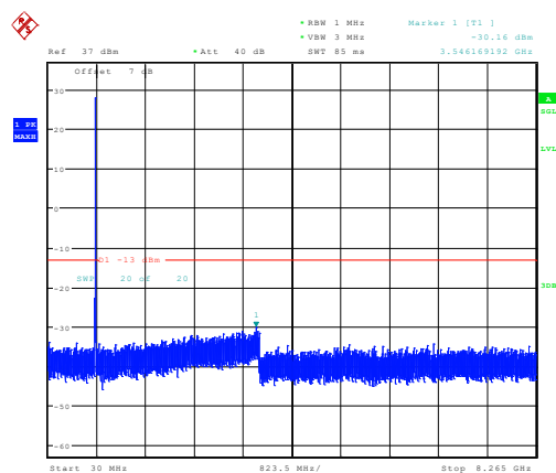
5MHz_Low_QPSK_1@0 -30.16dBm
