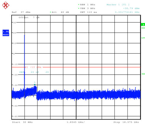
15MHz_Low_QPSK_1@0 -30.79dBm
