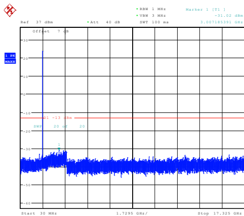
10MHz_Middle_QPSK_1@0 -31.02dBm
