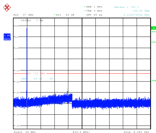
5MHz_Middle_QPSK_1@0 -30.42dBm
