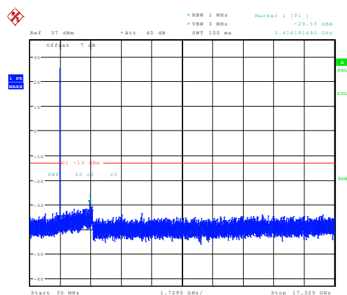
5MHz_Middle_QPSK_1@0 -29.53dBm
