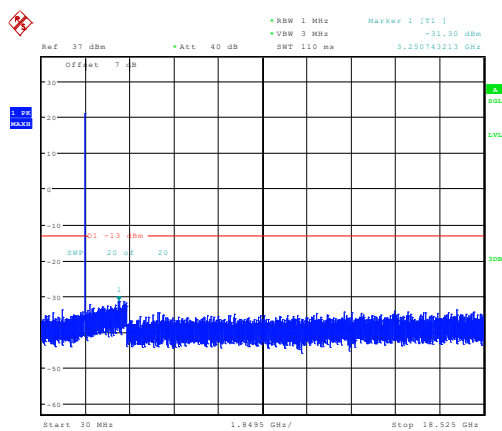
5MHz_Low_QPSK_25@0 -31.30dBm
