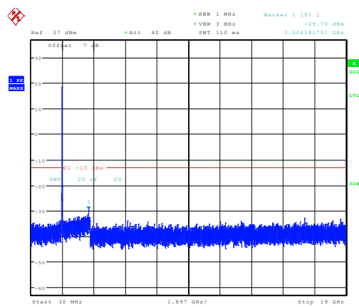
20MHz_High_QPSK_1@0 -29.70dBm
