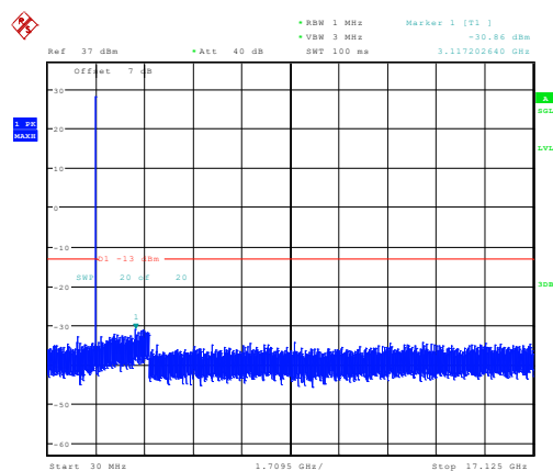
5MHz_Low_QPSK_1@0 -30.86dBm
