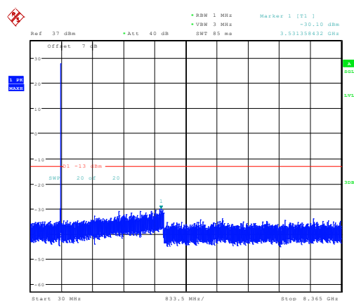
3MHz_Middle_QPSK_1@0 -30.10dBm
