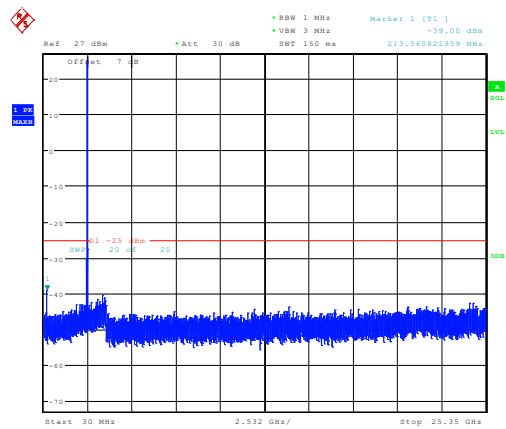
15MHz_Middle_QPSK_1@0 -39.00dBm
