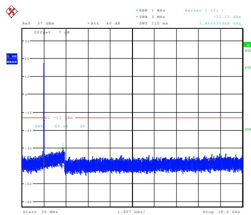
20MHz_Low_QPSK_100@0 -31.15dBm
