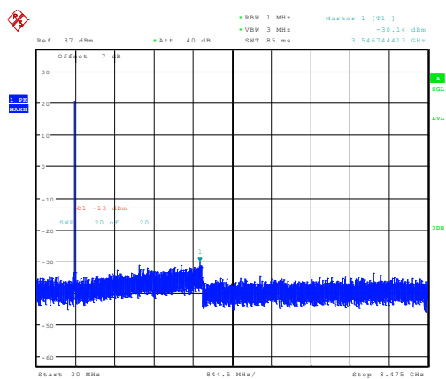
3MHz_High_QPSK_15@0 -30.14dBm
