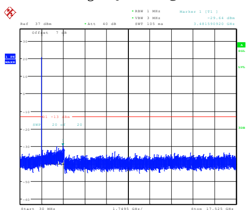
5MHz_High_QPSK_25@0 -29.64dBm
