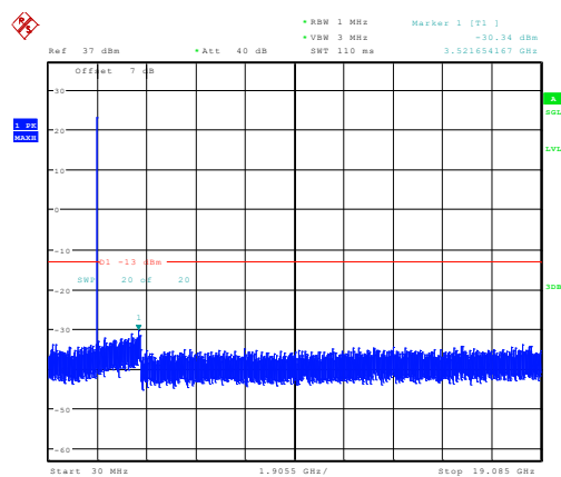
3MHz_High_QPSK_1@0 -30.34dBm
