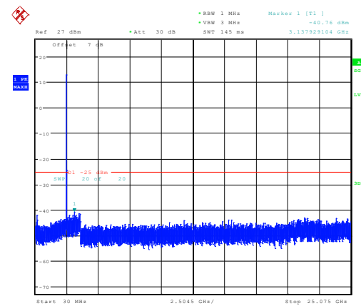
15MHz_Low_QPSK_75@0 -40.76dBm
