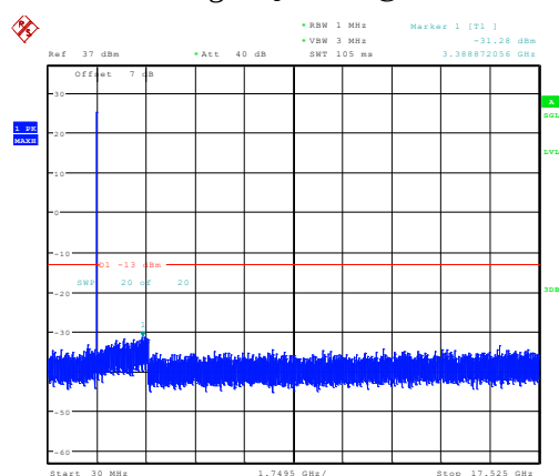
5MHz_High_QPSK_1@0 -31.28dBm
