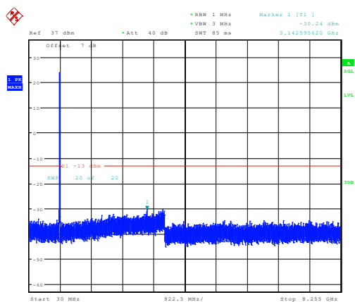
3MHz_Low_QPSK_15@0 -30.24dBm
