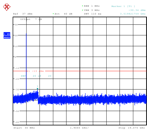
5MHz_High_QPSK_1@0 -30.34dBm
