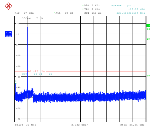
15MHz_Middle_QPSK_75@0 -37.55dBm
