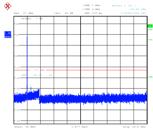
15MHz_Middle_QPSK_75@0 -30.80dBm
