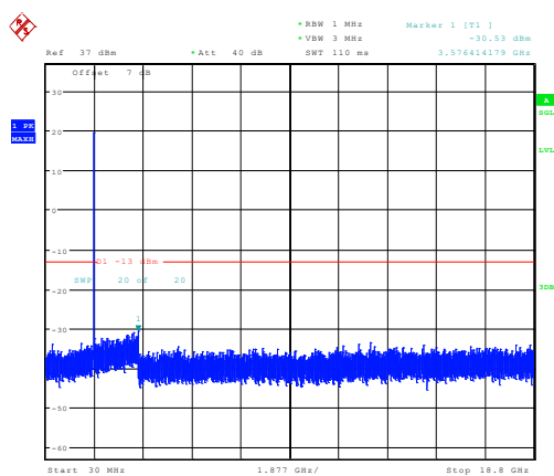
5MHz_Middle_QPSK_25@0 -30.53dBm
