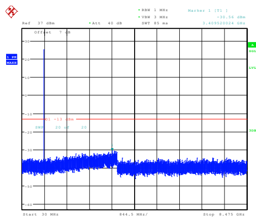
3MHz_High_QPSK_1@0 -30.56dBm
