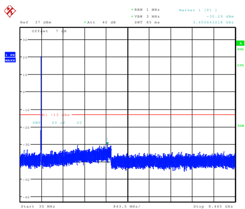
5MHz_High_QPSK_25@0 -30.29dBm
