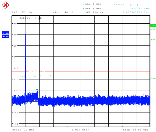
10MHz_High_QPSK_1@0 -30.62dBm
