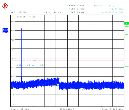
3MHz_Middle_QPSK_15@0 -30.97dBm
