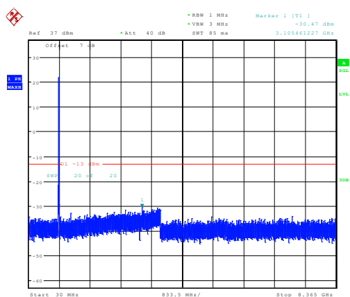
5MHz_Middle_QPSK_25@0 -30.47dBm
