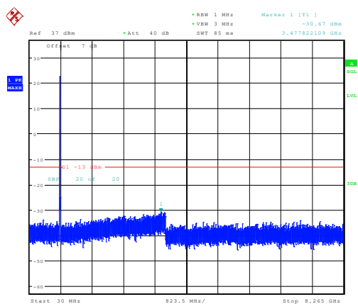
5MHz_Low_QPSK_25@0 -30.67dBm
