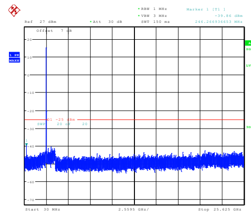
15MHz_High_QPSK_75@0 -39.86dBm
