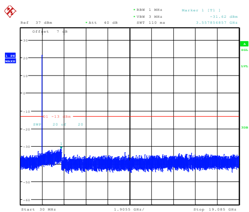
3MHz_High_QPSK_15@0 -31.62dBm
