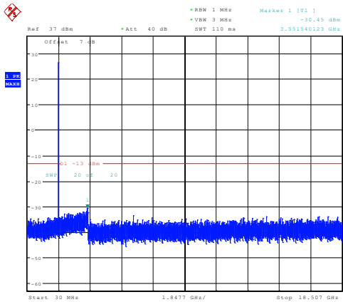
1.4MHz_Low_QPSK_6@0 -30.45dBm
