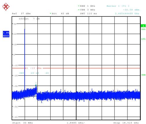
3MHz_Low_QPSK_15@0 -30.58dBm
