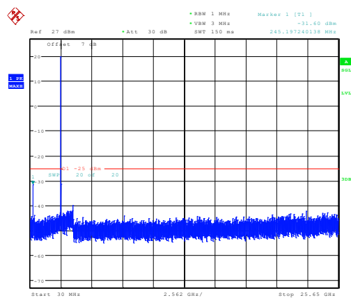
10MHz_High_QPSK_1@0 -31.60dBm
