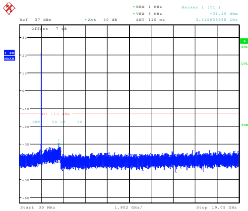
10MHz_High_QPSK_50@0 -31.15dBm
