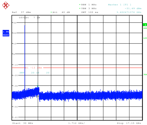
10MHz_Low_QPSK_1@0 -31.49dBm
