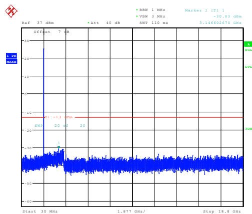
3MHz_Middle_QPSK_1@0 -30.83dBm
