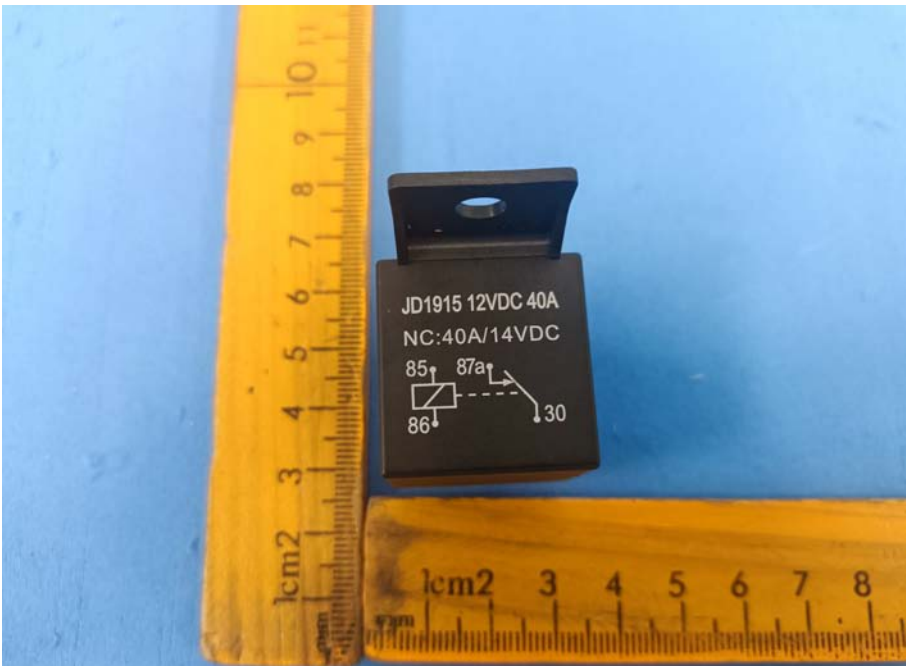
Cut Relay
