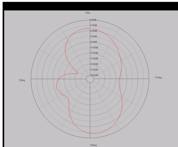
H plane
