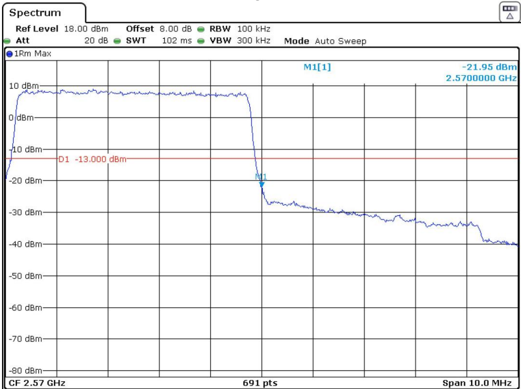
Band 7_5 MHz_High_16QAM_RB25#0
