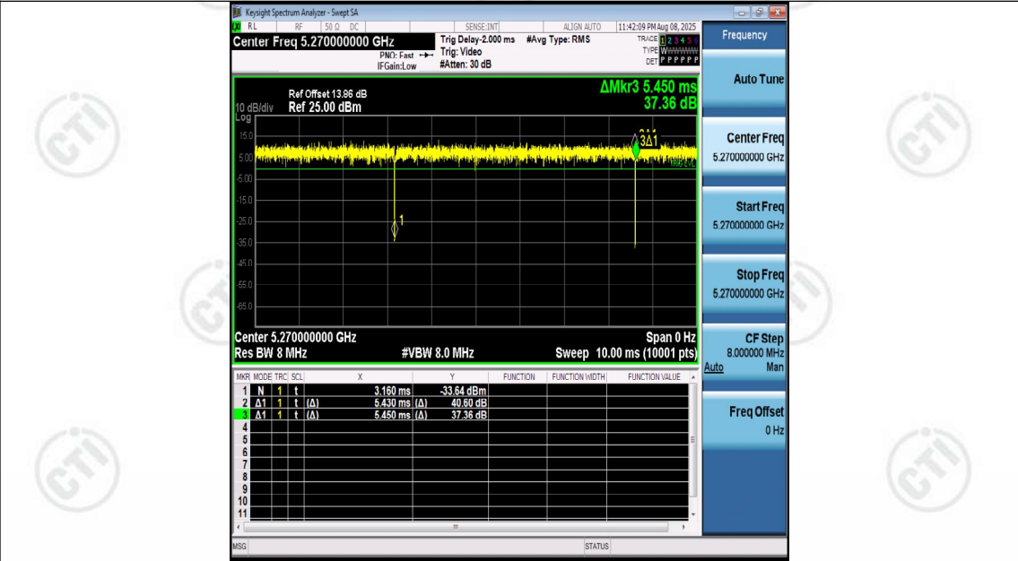
NTVN-11N40MIMO-Ant1-5270
