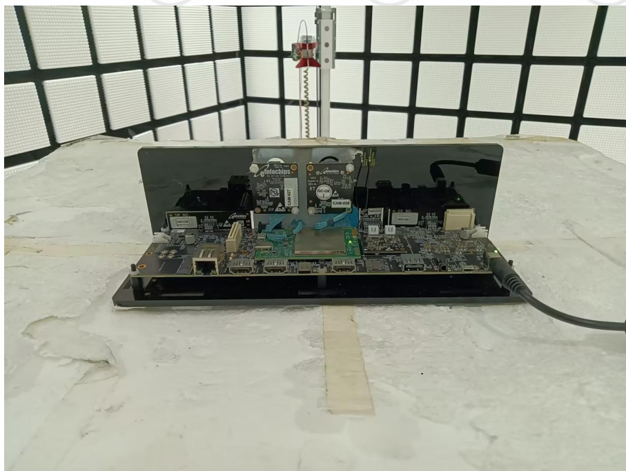
Radiated spurious emission Test Setup-2(Above 18GHz)
