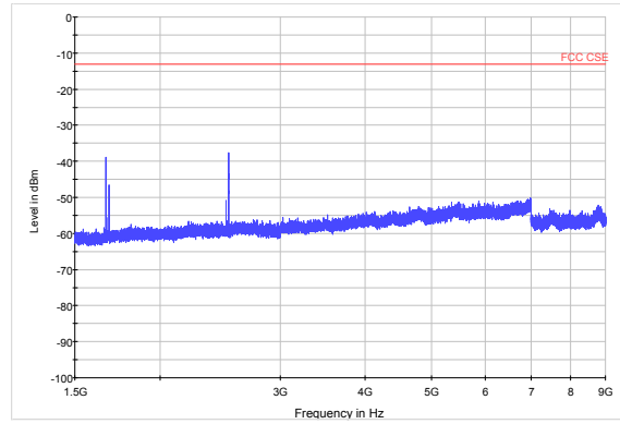
LTE Band 26 10MHz CH-High 1.5GHz~9GHz
