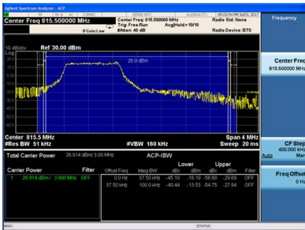
LTE Band 26 16QAM 100%RB CH Low 3M
