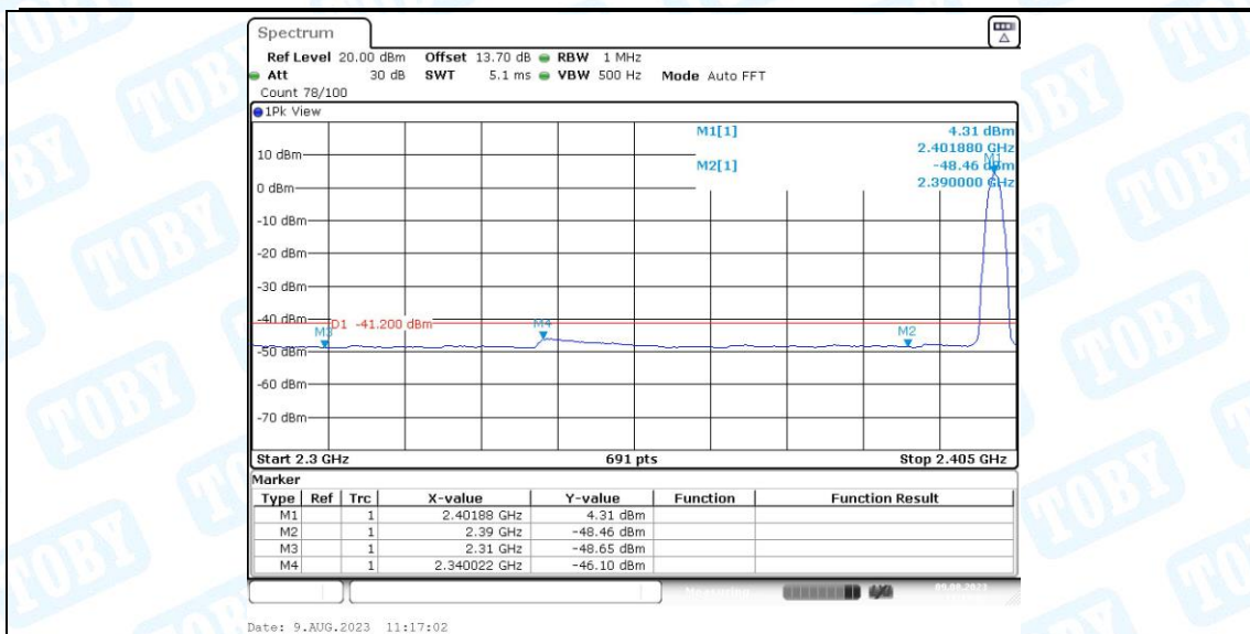
2DH5_Ant1_Low_2402_Peak
