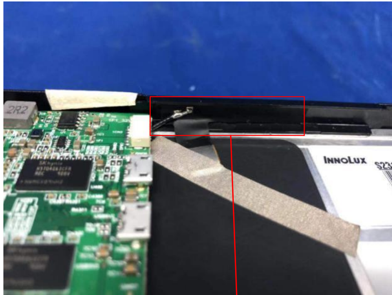
RF Antenna
