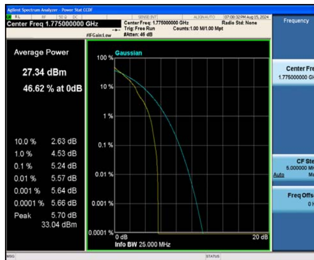
Band66-10MHz-QPSK-132622-50RB#0
