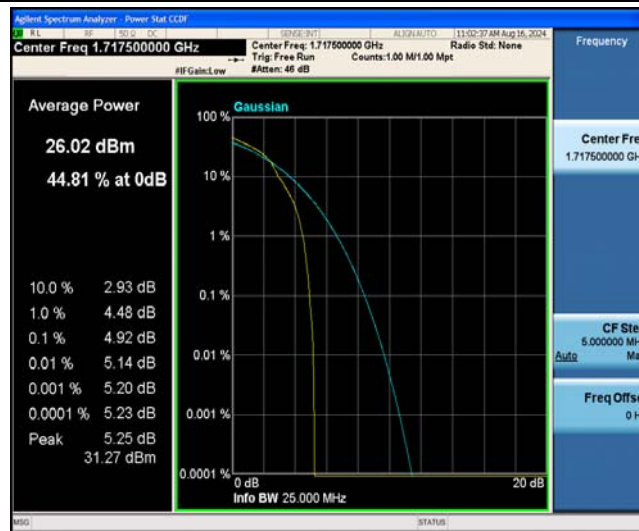
Band66-15MHz-16QAM-132047-27RB#0
