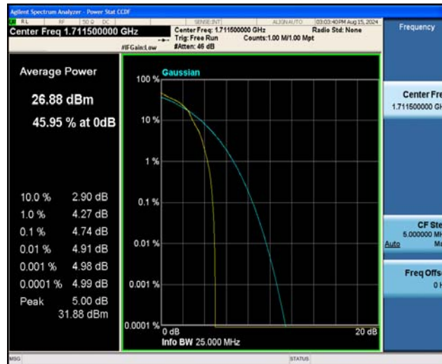
Band66-3MHz-16QAM-131987-15RB#0
