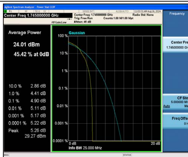
Band66-15MHz-16QAM-132322-27RB#0
