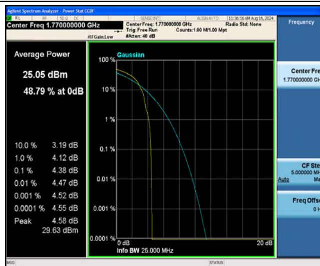
Band66-20MHz-16QAM-132572-27RB#0
