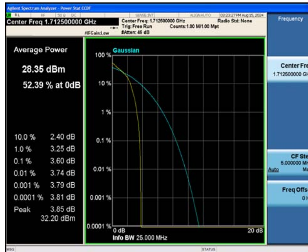
Band66-5MHz-QPSK-131997-25RB#0
