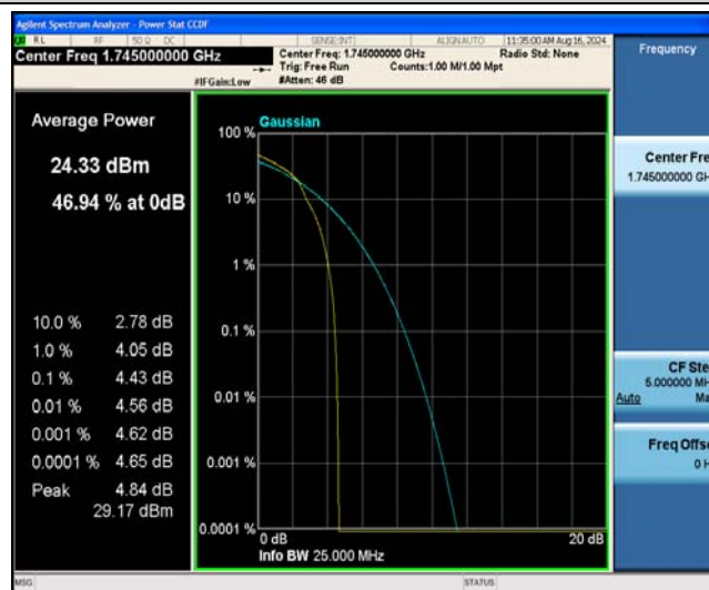
Band66-20MHz-16QAM-132322-27RB#0
