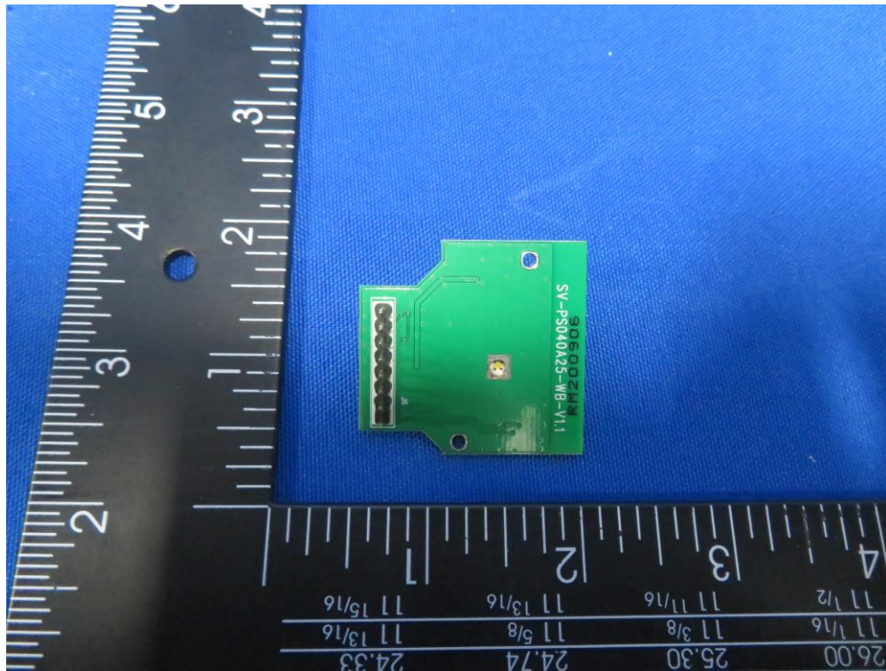
(11) EUT Photo
