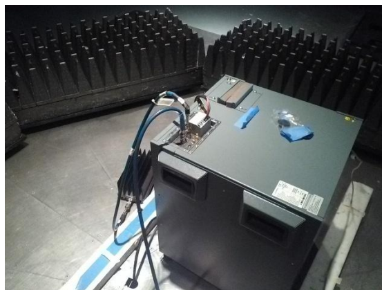
Output power, bandwidth, adjacent channel measurement
