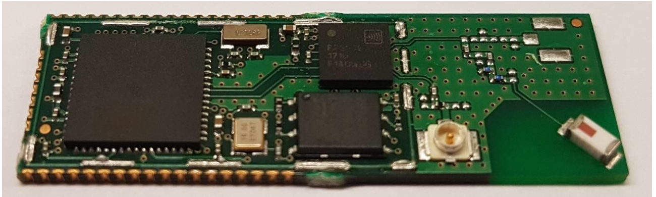
EUT 2.4 GHz radio module unshielded
