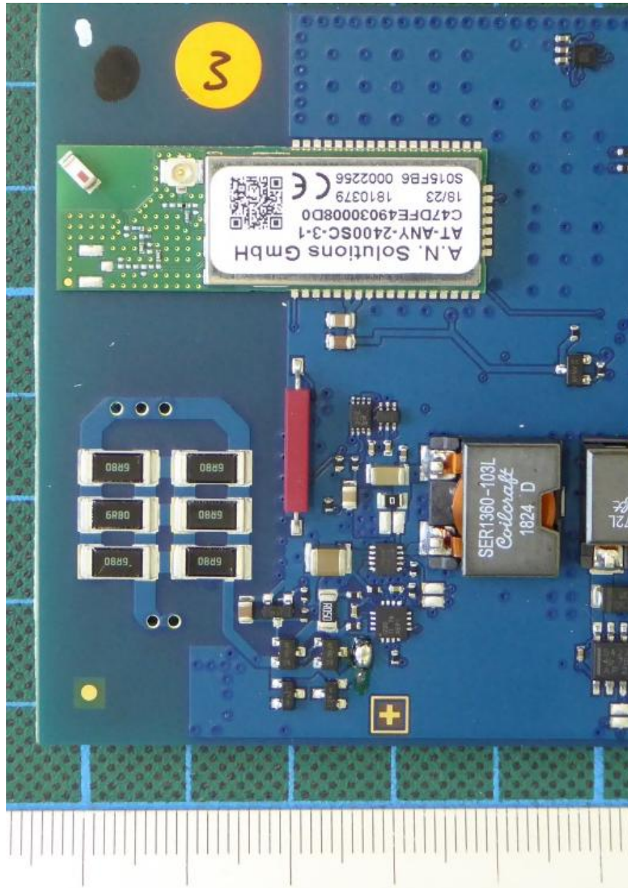
EUT 2.4 GHz radio module Detail view
