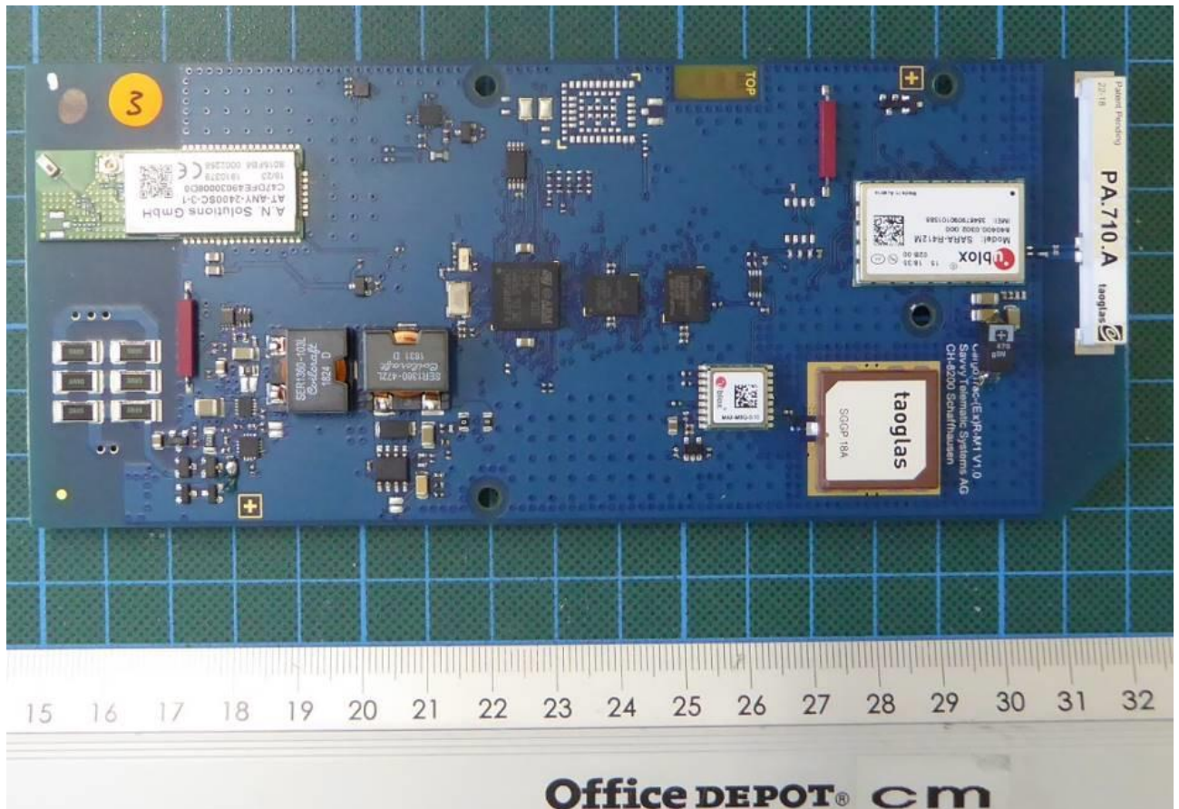
EUT PCB Top view
