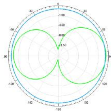
Gain Plot 2
