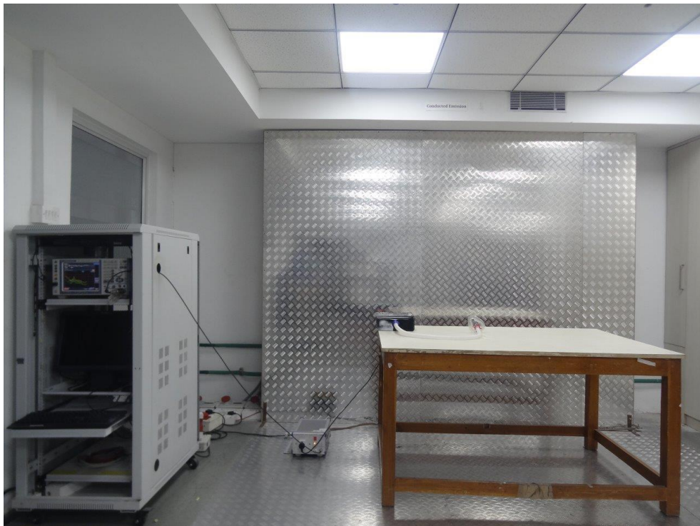
CE Testing Test setup
