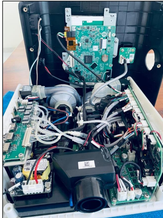
COUGH_DEVICE_ASSEMBLY
