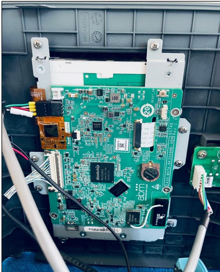
CLEAR_TOP_ASSEMBLY
