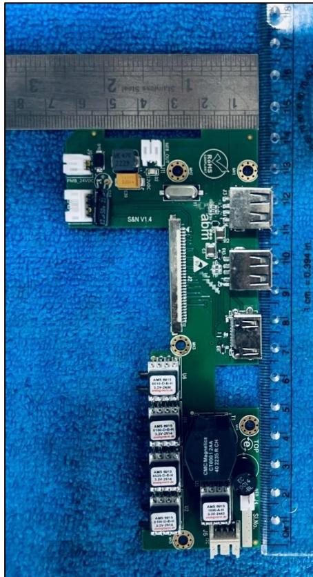
CLEAR_SENSOR_MEASUREMENT
