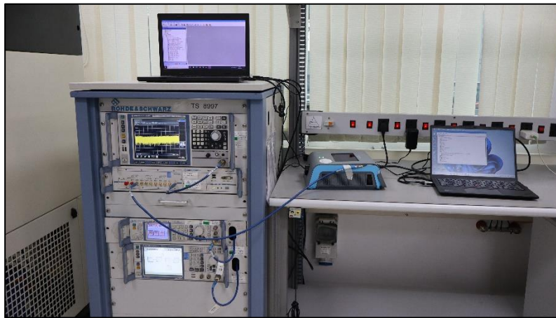
BLE Conducted Test Setup
