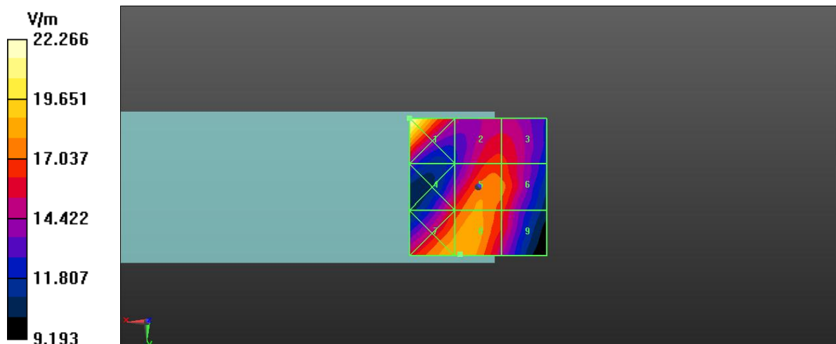
Fig A.9 HAC RF E-Field LTE Band 38
