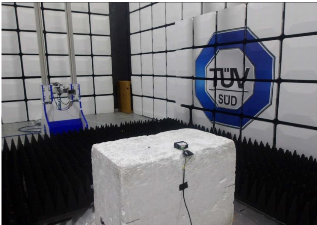
Figure 4 - Radiated Emission (8GHz to 13GHz)
