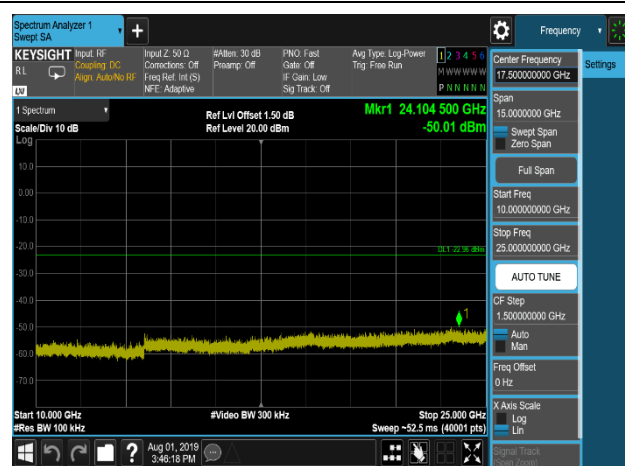
DQPSK,2480MHz,2DH5,Plot 4,10000MHz~25000MHz
