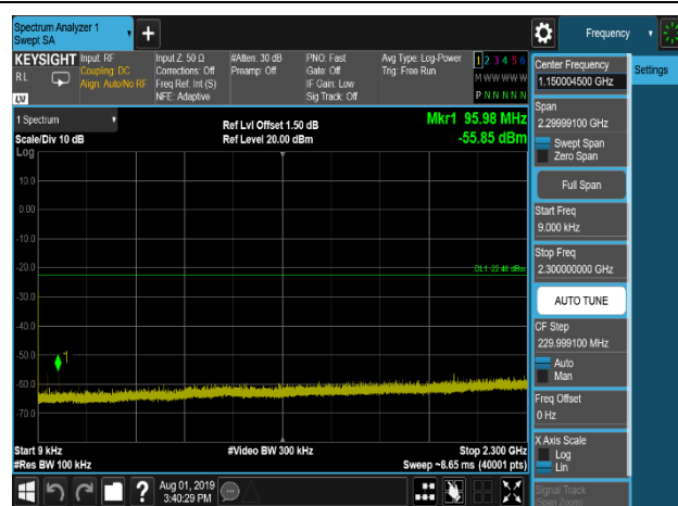
DQPSK,2441MHz,2DH5,Plot 2,0.009MHz~23 00MHz
