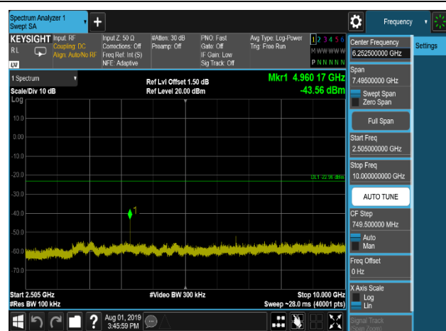
DQPSK,2480MHz,2DH5,Plot 3,2505MHz~10000MHz
