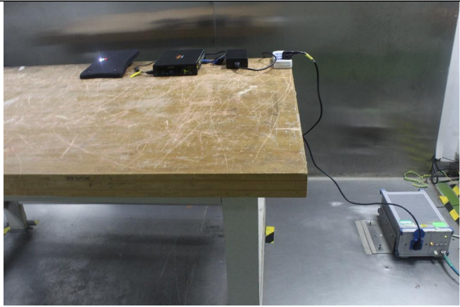
Conducted emission
