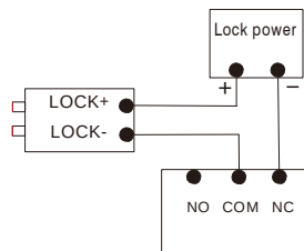
Switching Value Output: Normally-closed connection
