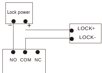
Switching Value Output: Normally-open connection
