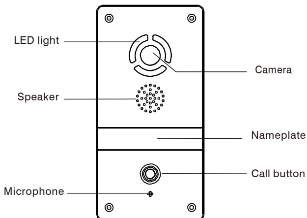
Model: 280SD-C12(with nameplate)
