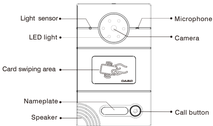
Model: 280SD-C3(with card)
