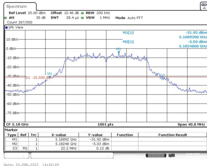
11AC20SISO_Ant2_5180
