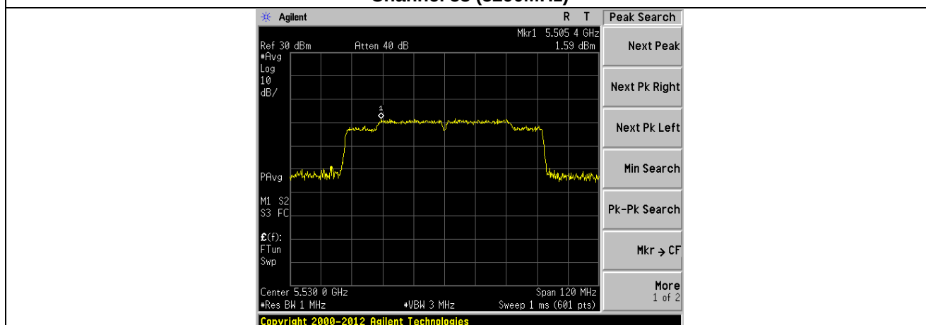
Channel 58 (5530MHz)
