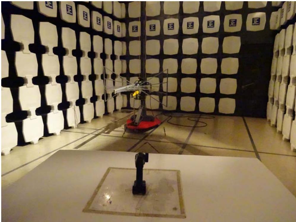
Measurement of Radiated Emission Test Set Up (30Hz – 1000MHz)
