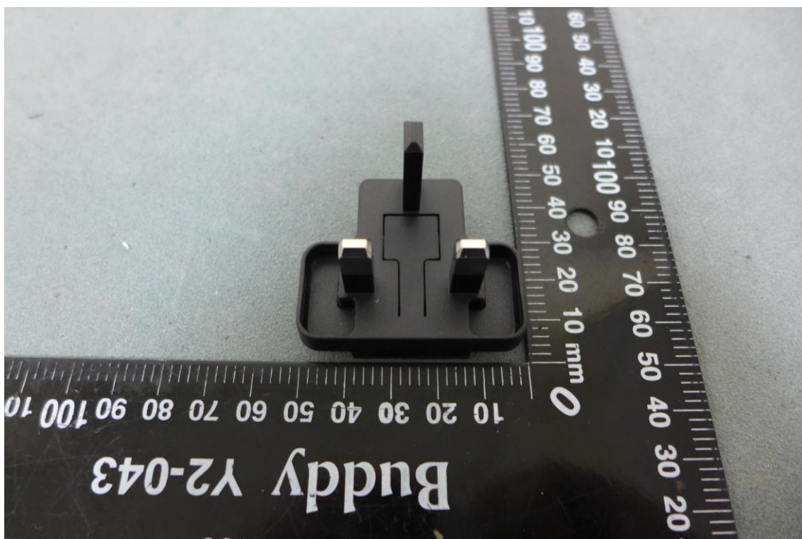
UK plug
