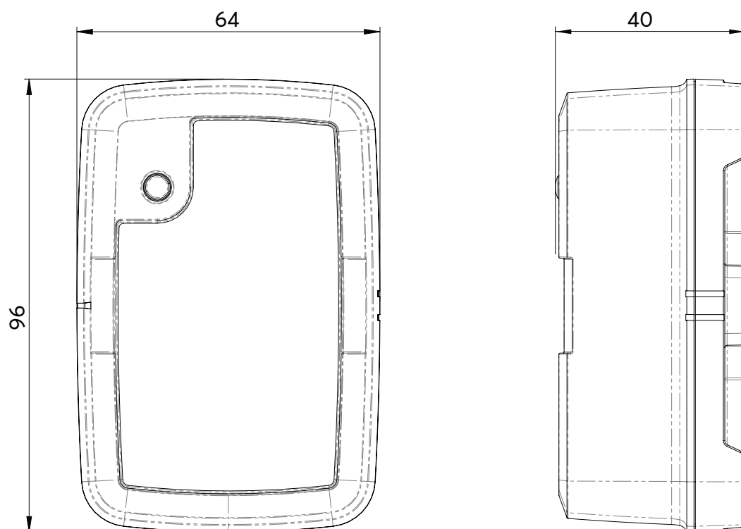
Fig. 1: Product dimensions
