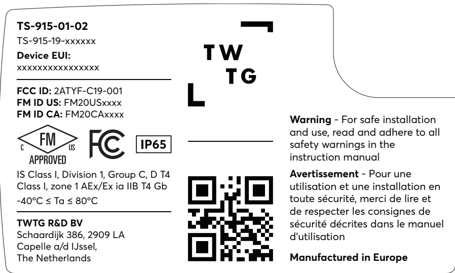
Fig. 2: Product label
