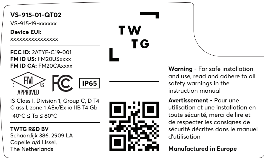
Fig. 2: Product label
