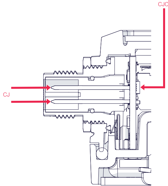
Figure 12: CJC Section Overview
