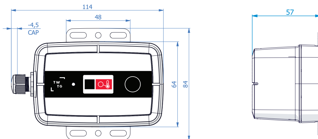
Figure 3: Neon Transmitter Dimensions (mm)
