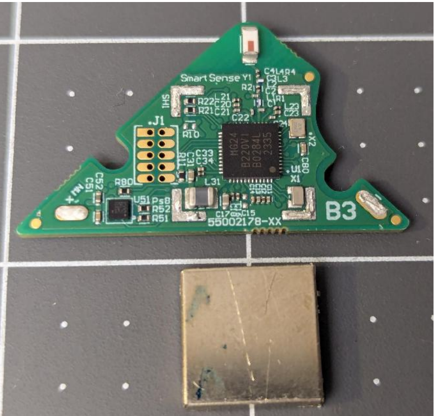
PCBA Top with RF Shield Removed
