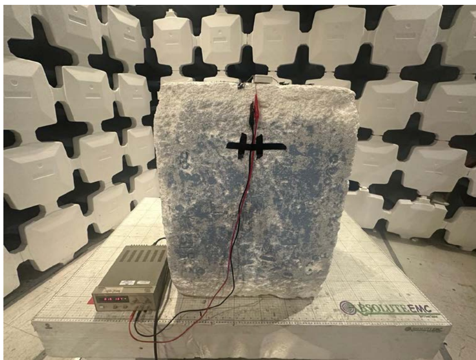
EUT Setup for radiated emissions
